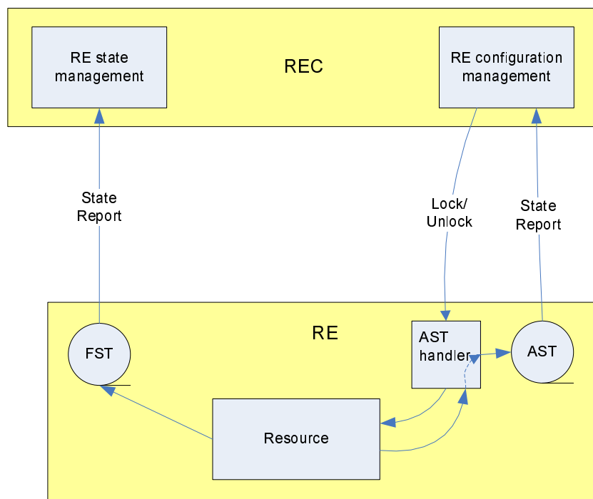
Figure 6.7.1.3-1: AST and FST relationship in RE and REC
