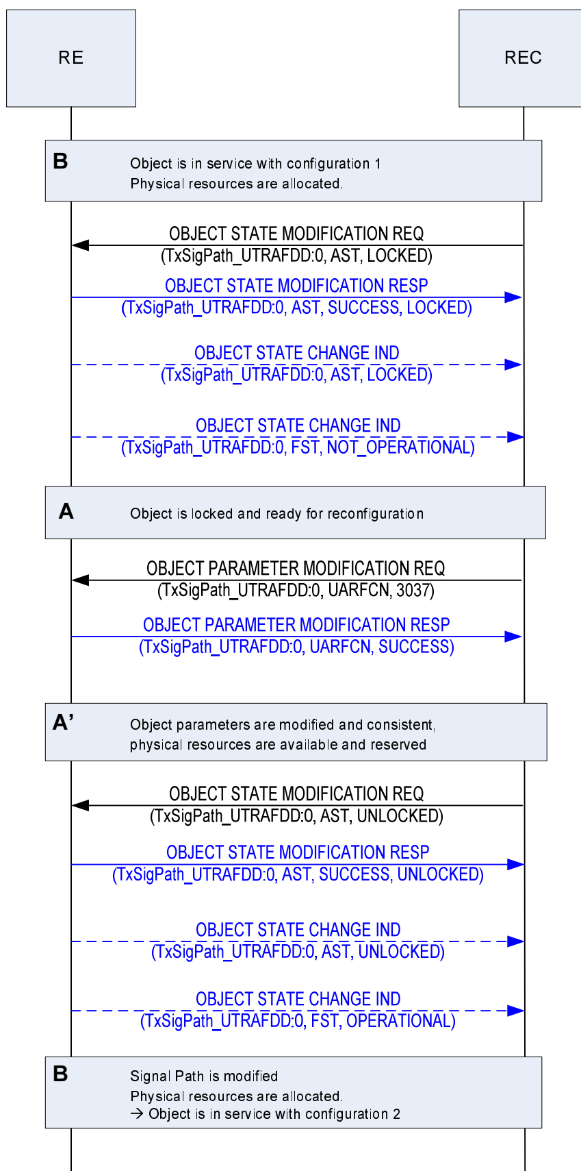
Figure 10.2.5.2-1: Sequence successful signal path modification
