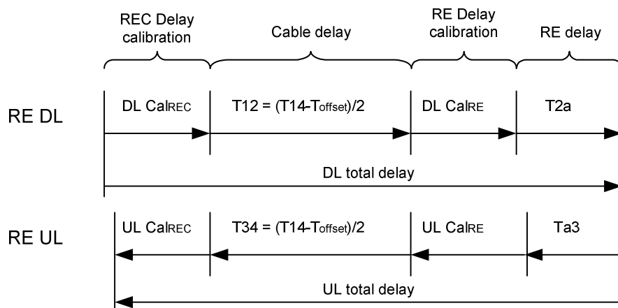
Figure 10.2.4-2: Relation of time components for single-hop
