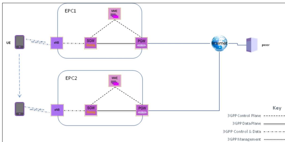
Figure 15: Model for UE moving across different EPC
