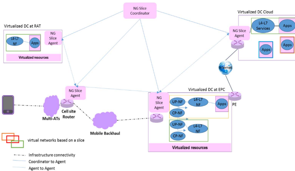
Figure 40: NG Slicing
