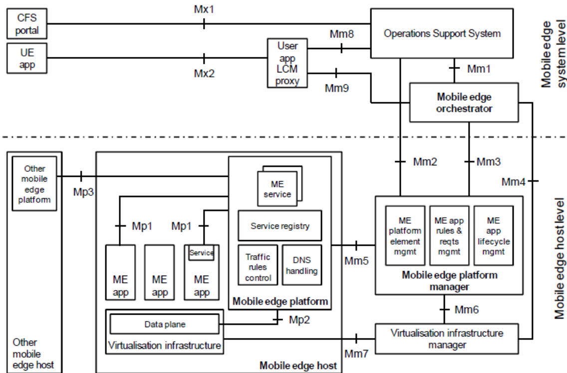
Figure 14: MEC Reference Architecture Framework (extracted from ETSI ETSI GS MEC 003 [20])
