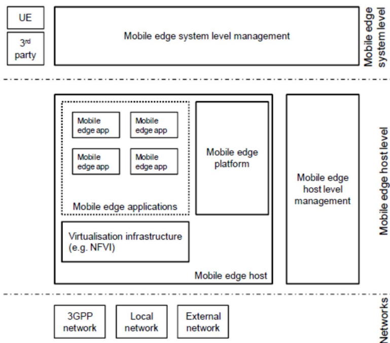
Figure 46: Mobile Edge Computing Framework, from reference [35]
