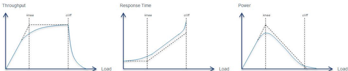
Figure 36: Congestion Curves
