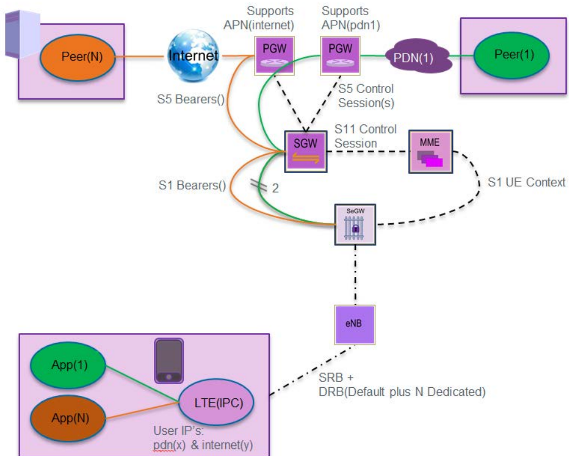
Figure 27: Release 12 LTE Access Network Support
