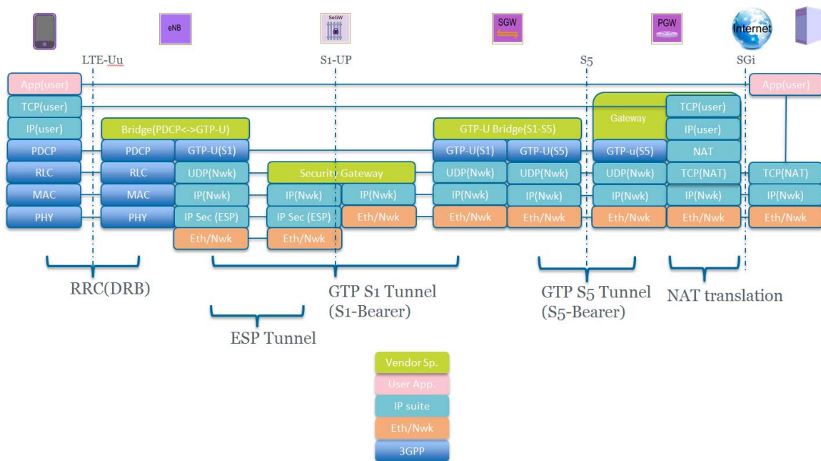
Figure 2: 3GPP LTE Rel-12 UP Protocols
