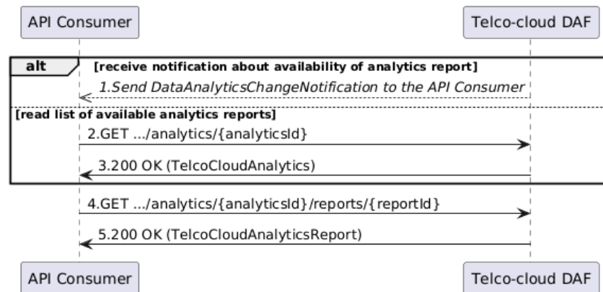
Figure 5.4.4-1: Flow of obtaining Telco-cloud data analytics reports
