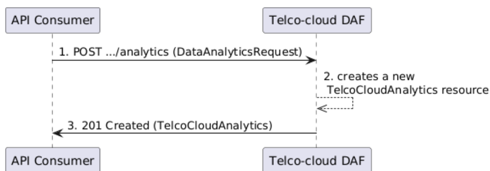
Figure 5.4.1-1: Flow of Data analytics creation
