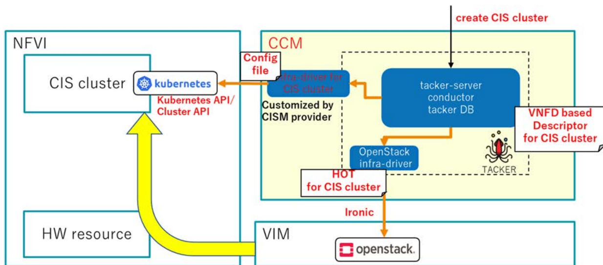
Figure A.5.4.4-1: Creation of bare-metal CIS cluster by OpenStack® Tacker
