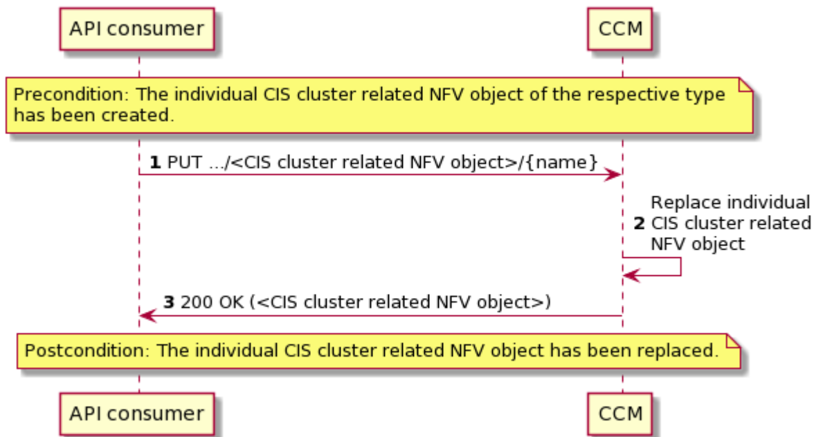
Figure 6.4.4.2-1: Flow of replacing a CIS cluster related NFV object
