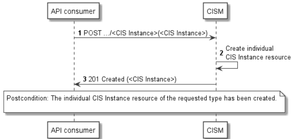
Figure 14.4.2-1: Flow of CIS Instance creation
