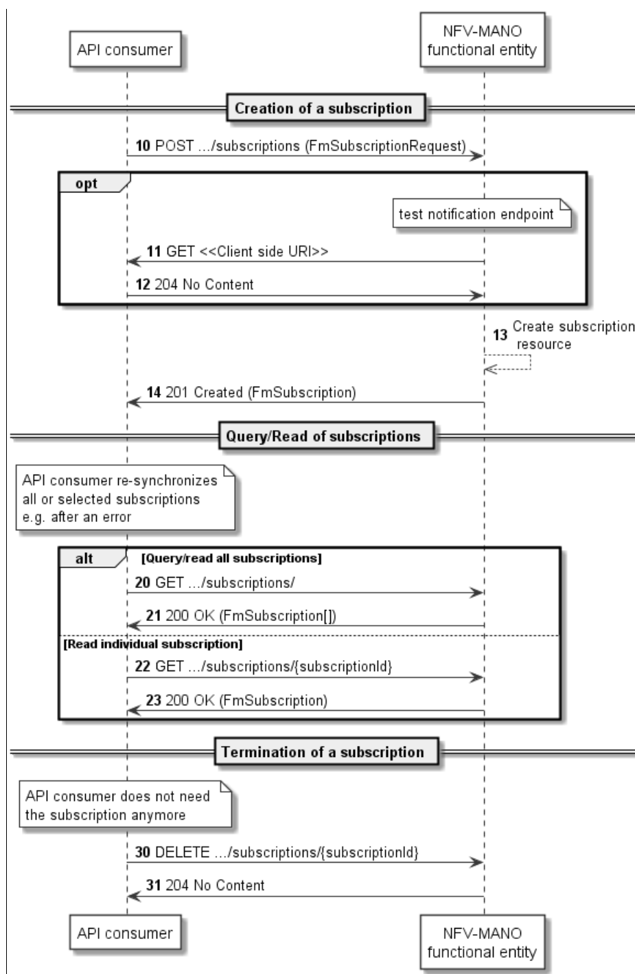
Figure 7.4.3-1: Flow of managing subscriptions
