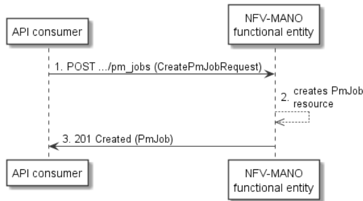
Figure 6.4.1-1: Flow of PM job creation
