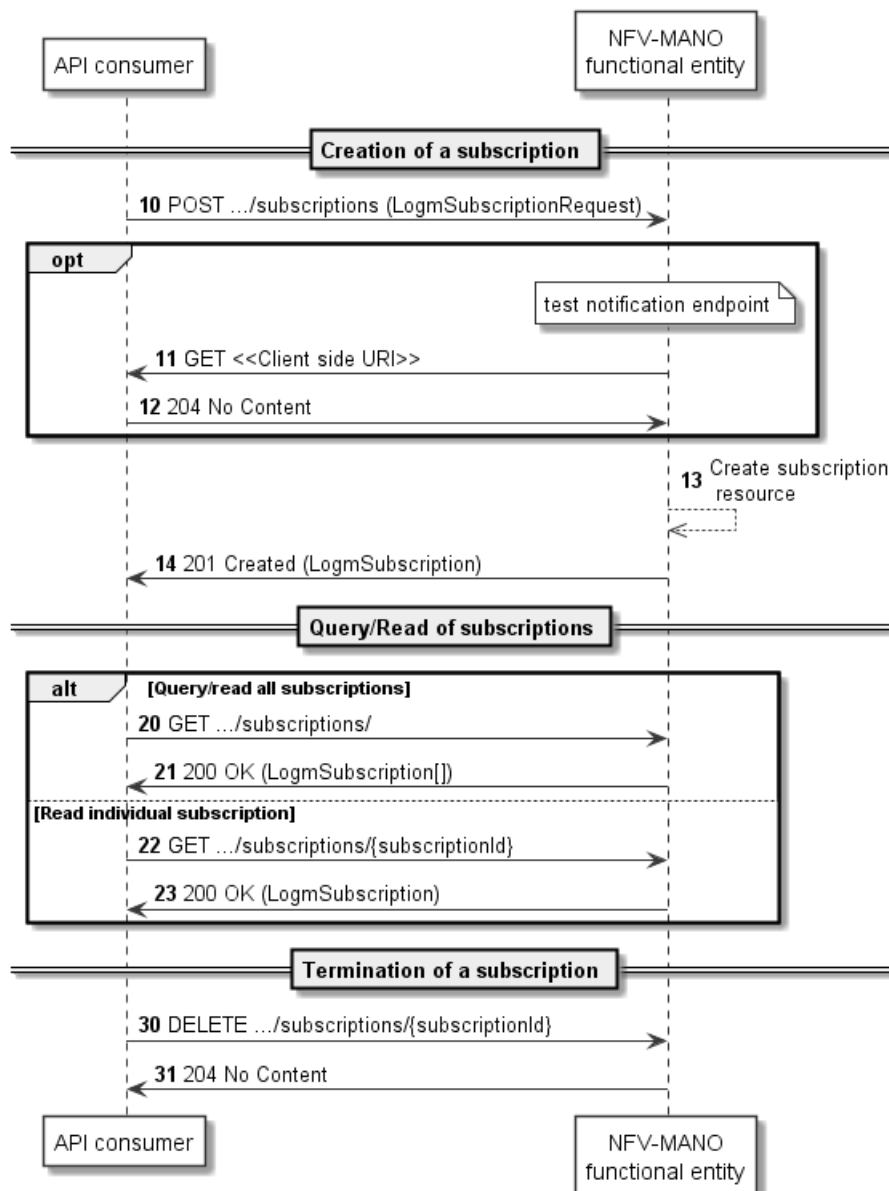
Figure 8.4.5-1: Flow of managing subscriptions
