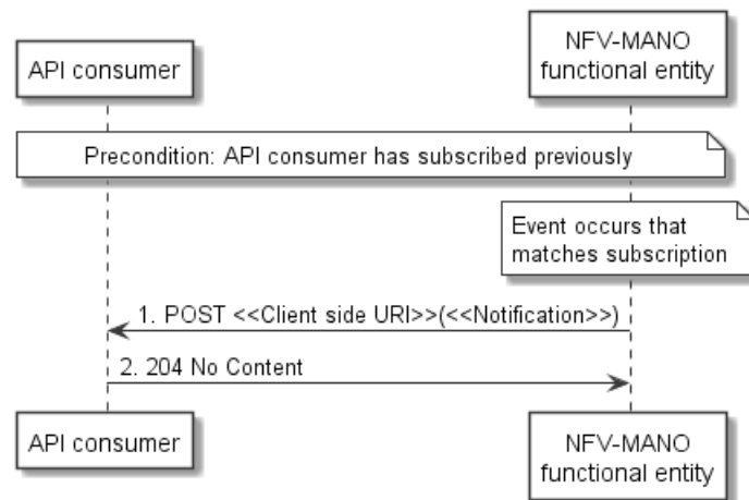
Figure 6.4.9-1: Flow of sending notifications
