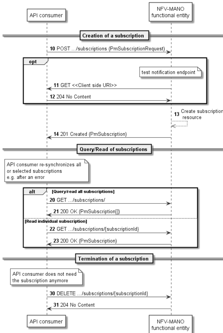
Figure 6.4.8-1: Flow of managing subscriptions
