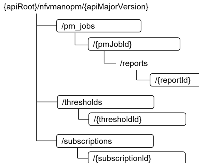
Figure 6.3-1: Resource URI structure of the NFV-MANO performance management interface
