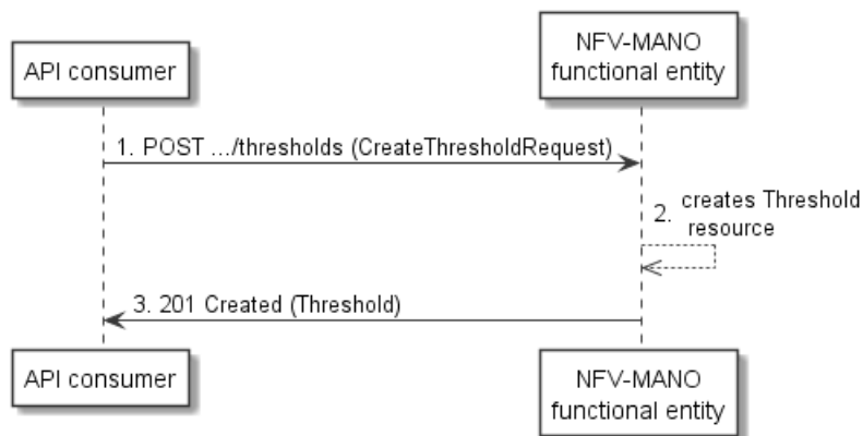
Figure 6.4.5-1: Flow of threshold creation
