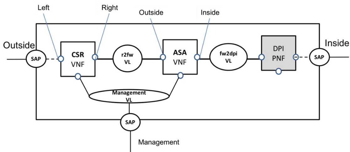
Figure A.2-2: Router Firewall DPI example
