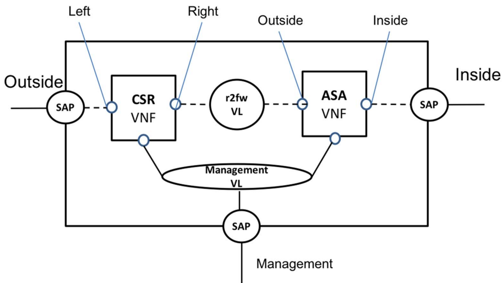
Figure A.2-1: Firewall Router Example
