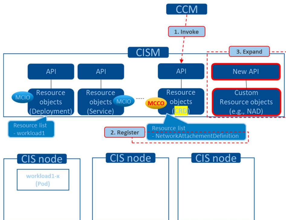
Figure C.1.2-1: Overview of applying MCCO for CCEC
