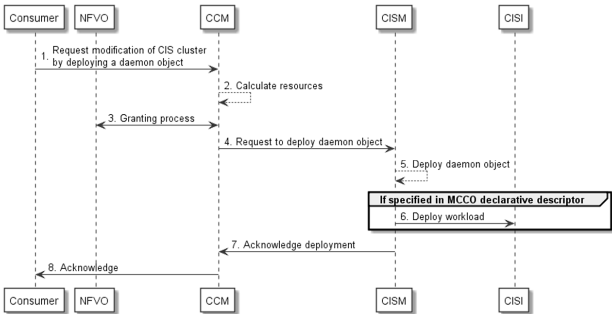
Figure B.5.5-1: Deploy daemon object on a CIS cluster
