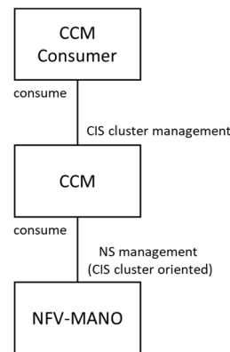
Figure 4.2.9-2: Relation of NS-based CIS cluster management and NS management
