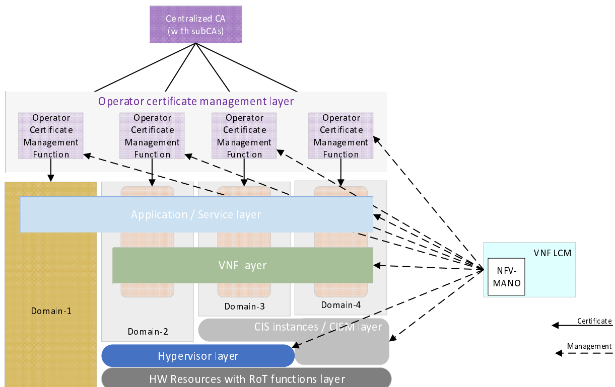
Figure 5.2.6-1: High-level view showing CA components
