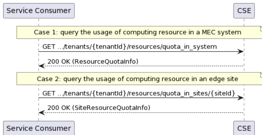
Figure 5.2.3.4-1: Flow of querying the computing resource quota
