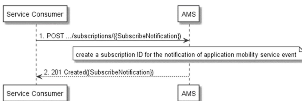
Figure 6.6-1: Flow of service consumer subscribing to notifications of Application Mobility Service events
