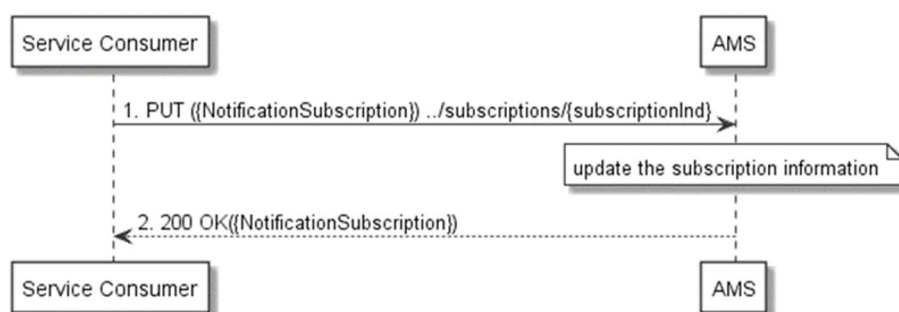
Figure 6.8-1: Flow of service consumer updating subscription to Application Mobility Service notifications
