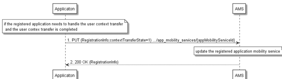
Figure 6.5-1: Flow of application instance sending the user context transfer completion notification
