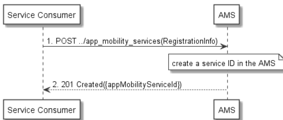
Figure 6.2-1: Flow of service consumer registration to AMS
