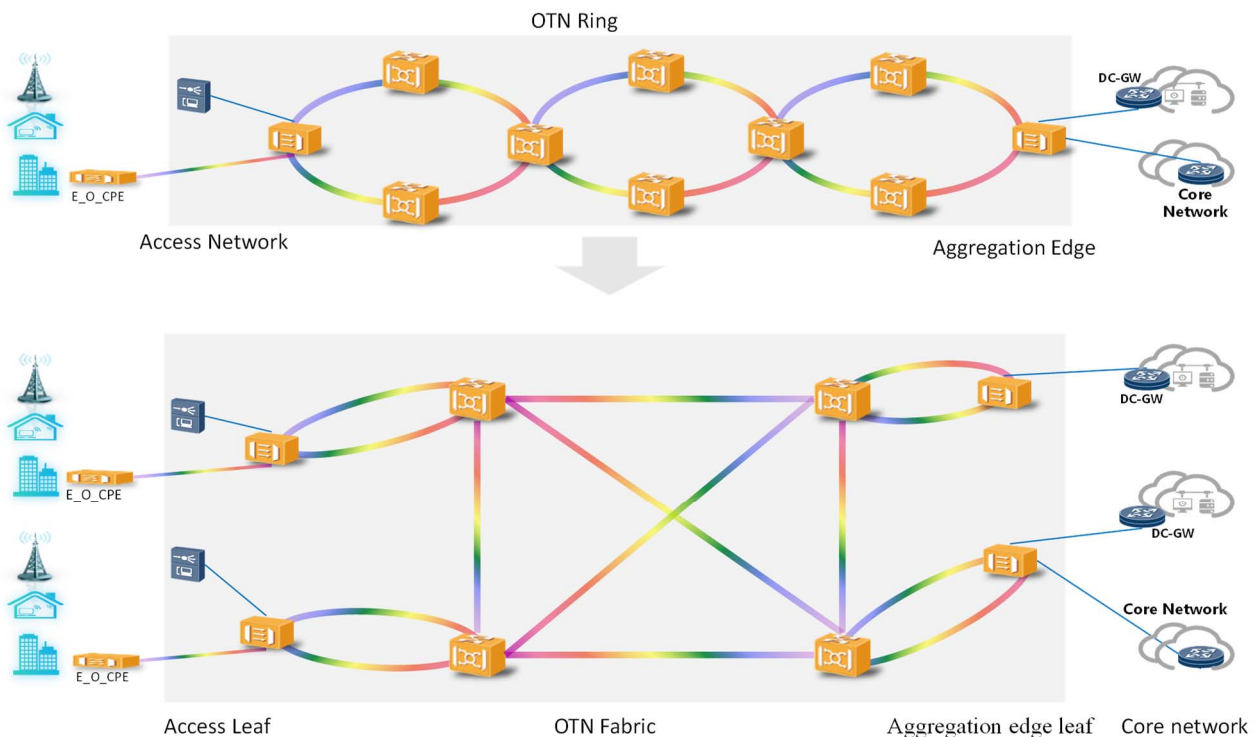
Figure 26: OTN Fabric
