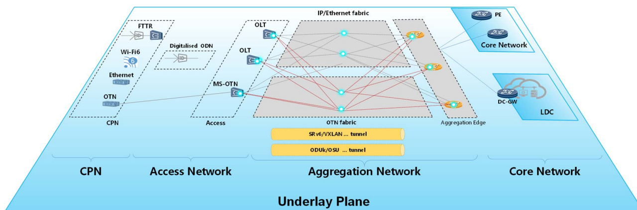
Figure 20: The functional blocks of the Underlay plane for F5G
