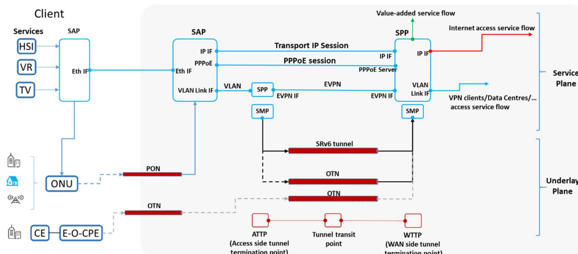
Figure 19: Example of Service-Network Separation for F5G
