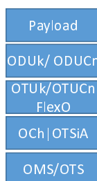
Figure 22: The OTN stack
