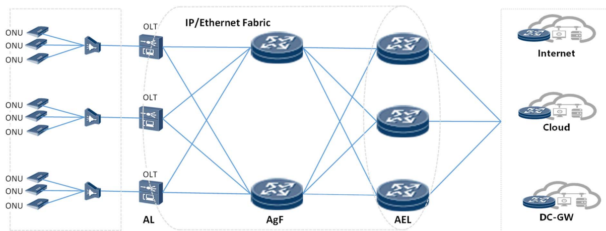
Figure 25: IP/Ethernet Fabric
