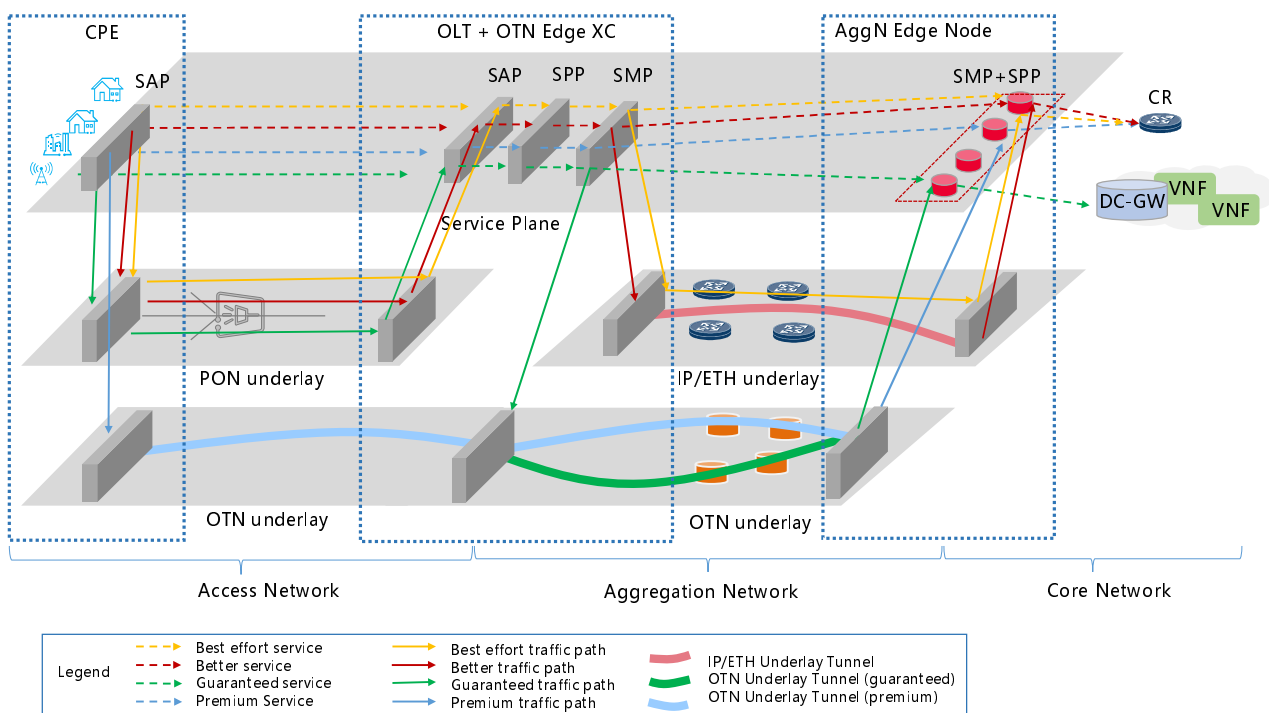
Figure 18: Example Traffic Steering Scenarios
