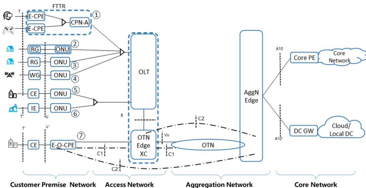
Figure 9: OTN control interfaces
