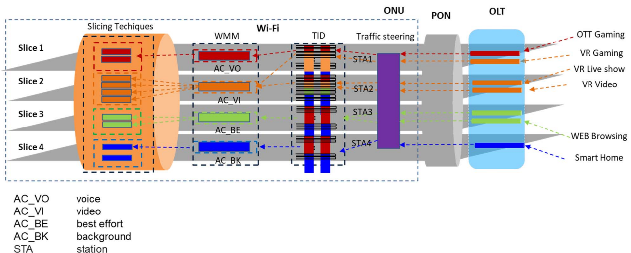
Figure 14: Overview for Wi-Fi Slicing
