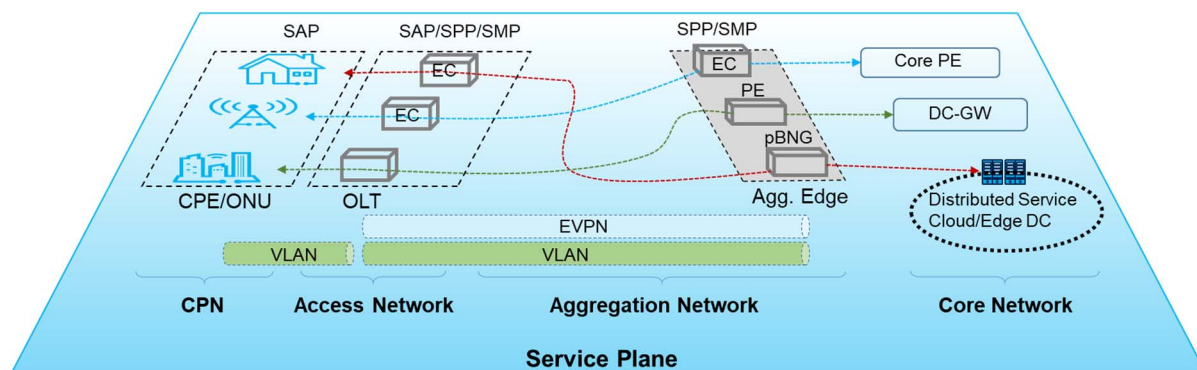
Figure 24: Functional blocks on the Service Plane for F5G
