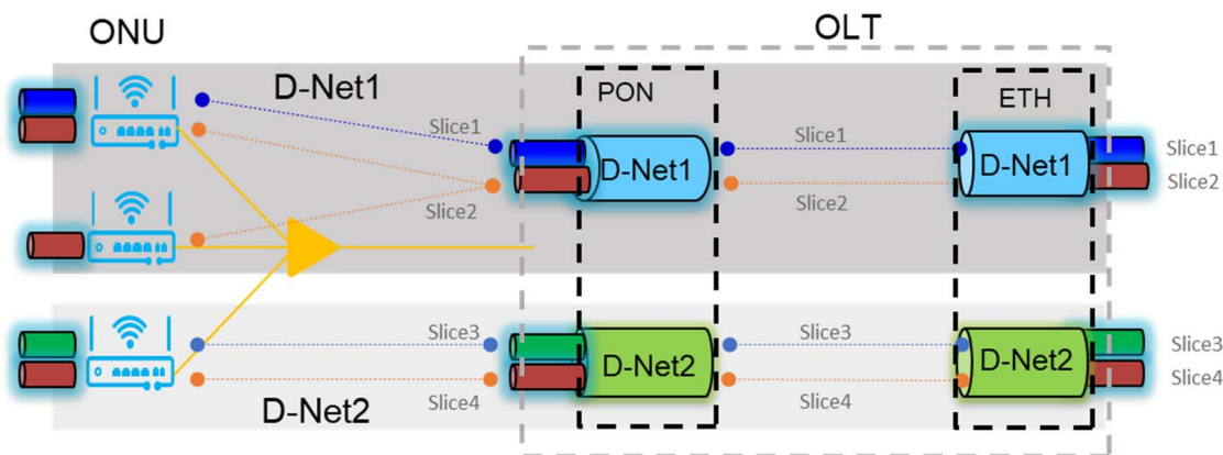
Figure 15: Overview for PON Slicing
