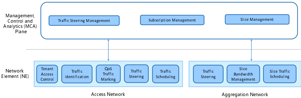
Figure 17: Traffic Steering Functional Overview
