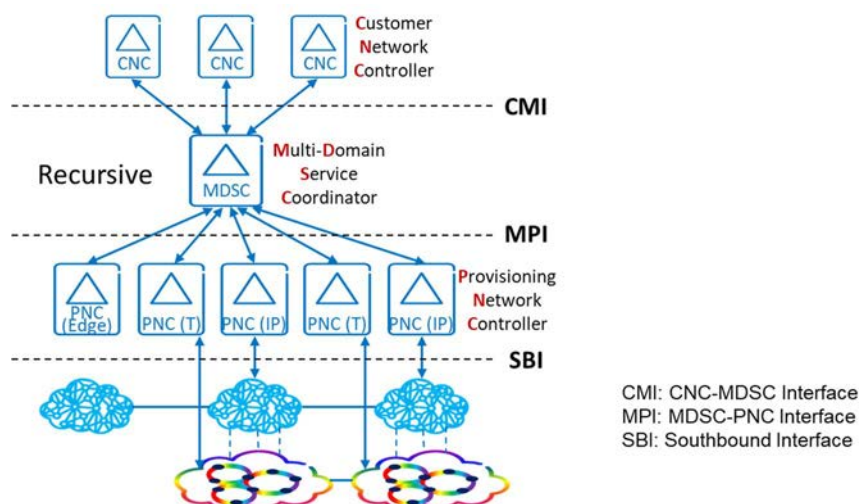
Figure 13: ACTN Architecture (Source: IETF RFC 8453 [1])
