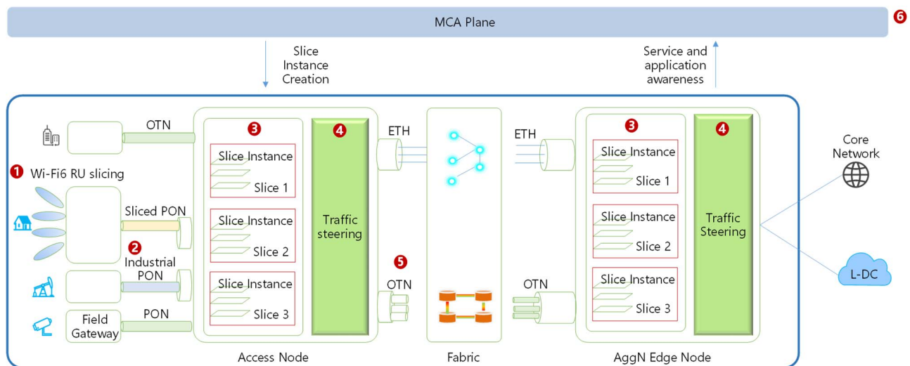
Figure 12: F5G Slicing Architecture
