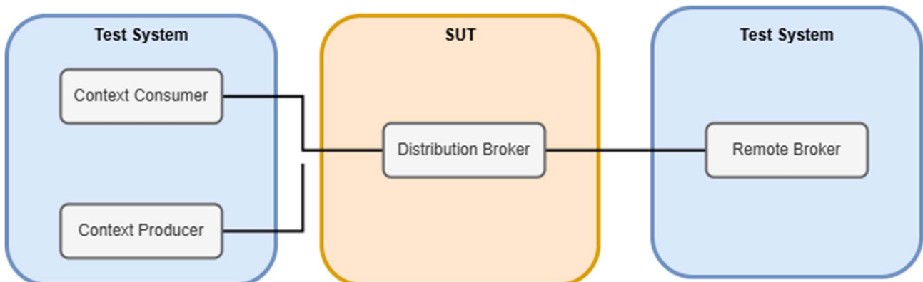
Figure 4.1-6: Test configuration 6 (CF_06)
