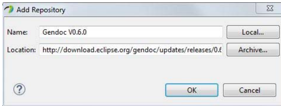
Figure 5.4-2: Installing Gendoc (2)
