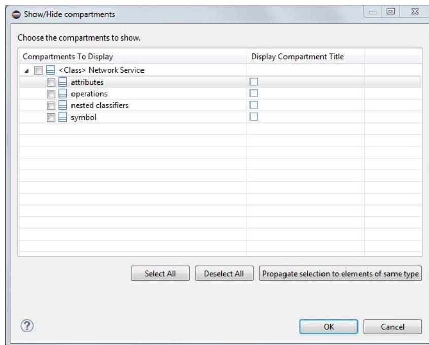
Figure 6.5-2: Hiding compartments (2)
