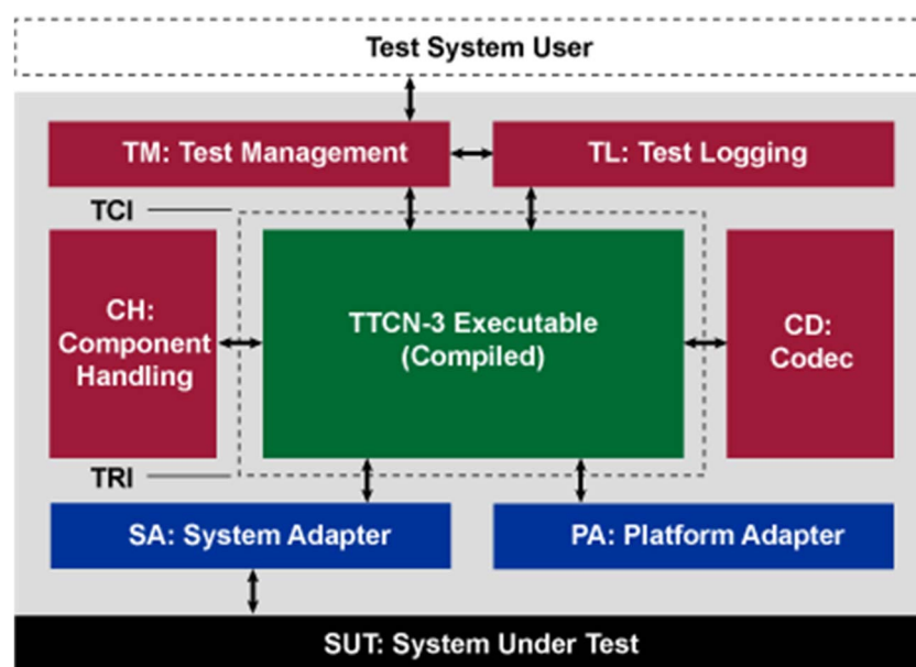
Figure 5.1.1-1: TTCN-3 elements
