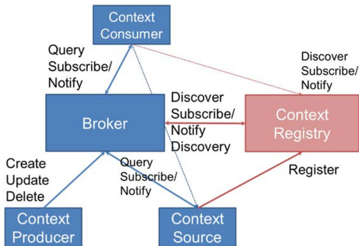
Figure 5.5-1: NGSI-LD architectural roles
