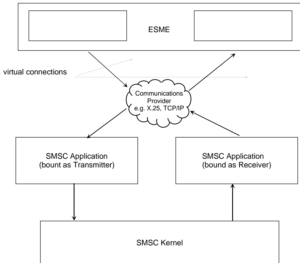
Figure A.4: ESME/SMSC Communication
