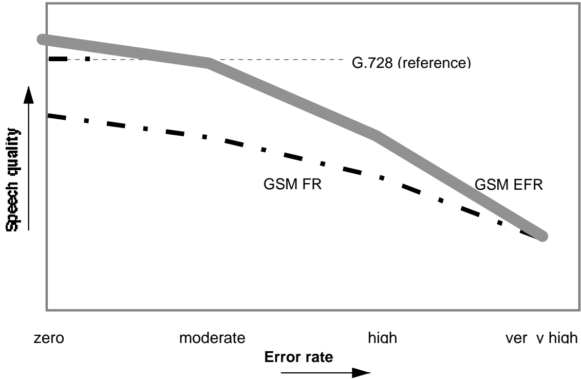
Figure 15: General trend of the EFR behaviour for error conditions in noise-free environment
