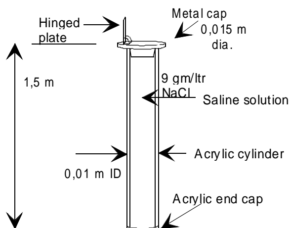
Figure 1: Typical saltwater column
