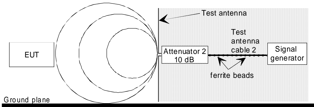
Figure 21: Stage 2: EUT measurement
