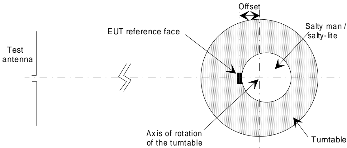
Figure 17: Illustration of offset from the axis of rotation
