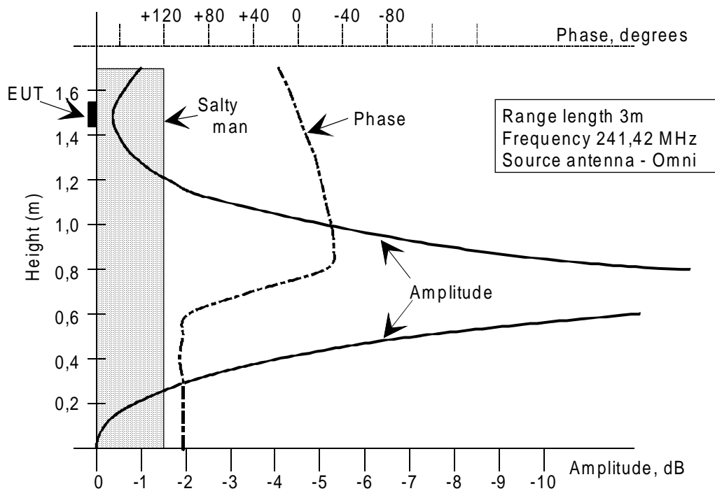
Figure 5: Amplitude and phase distribution along the Salty man over a reflective ground
