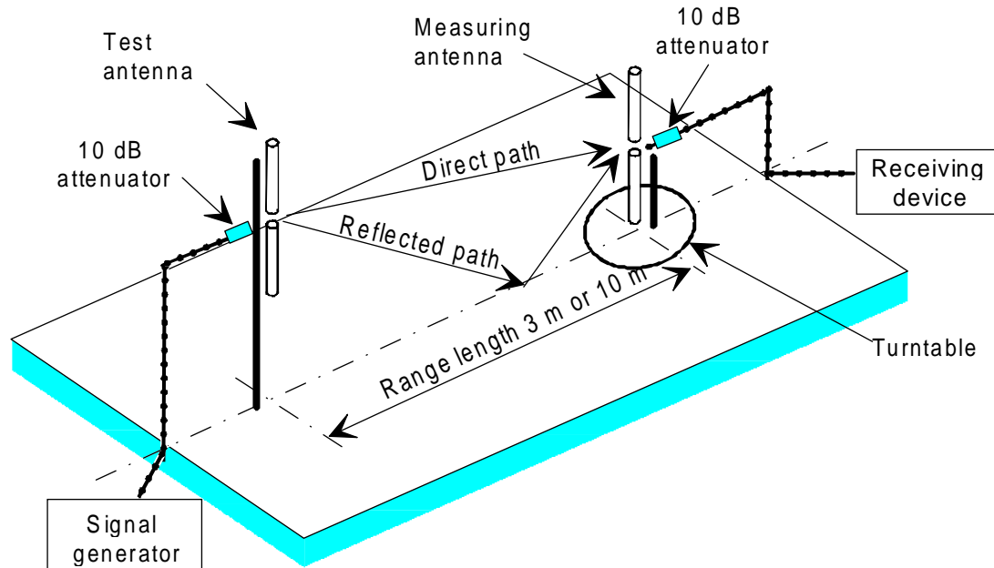
Figure 18: Equipment layout for the derivation of the transform factor during Sensitivity tests on an open area test site
