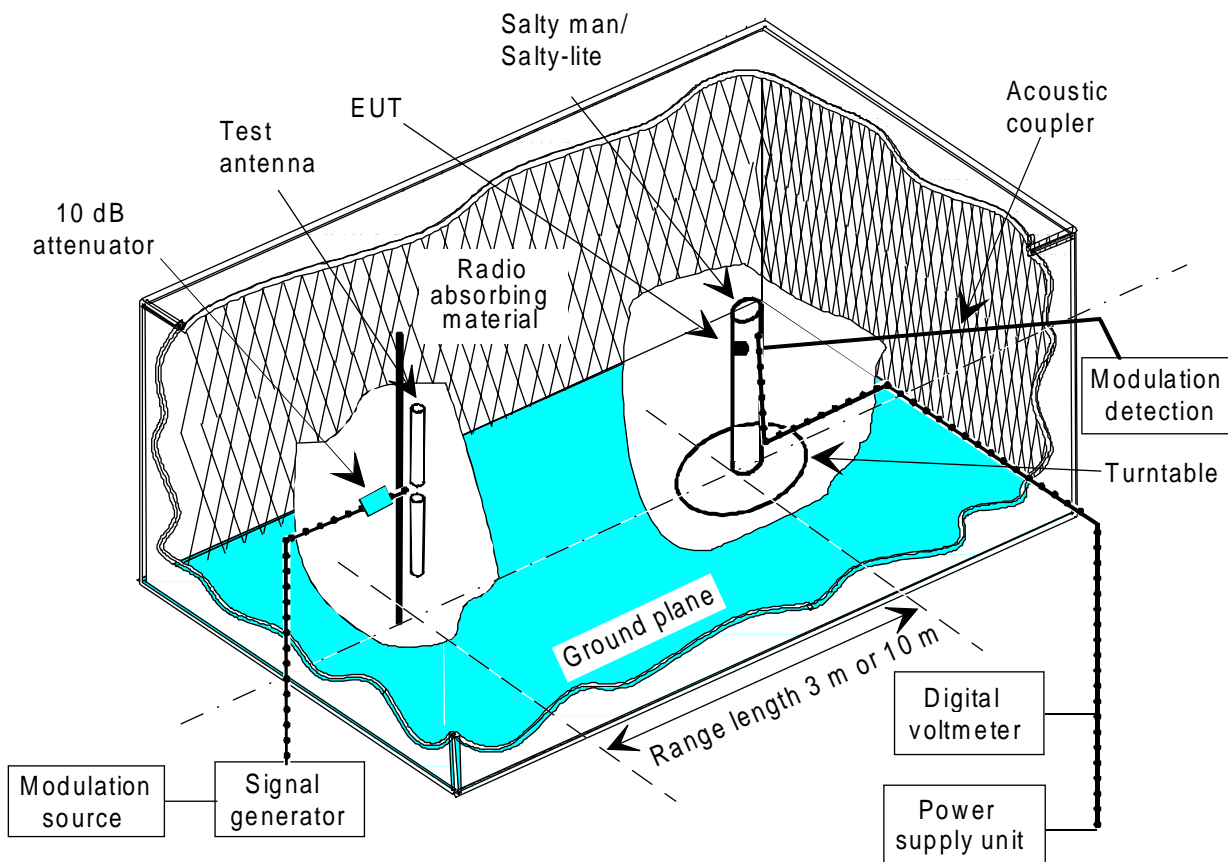
Figure 14: Anechoic chamber with a ground plane set-up for sensitivity tests on the EUT
