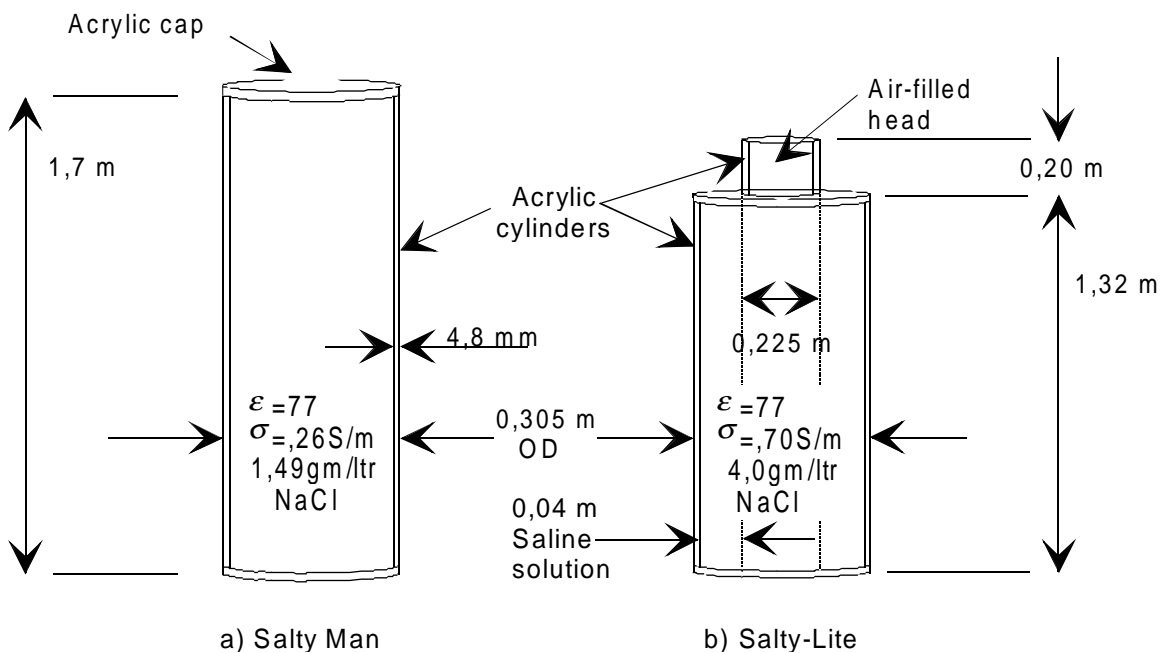
Figure 2: The two types of Salty man.
