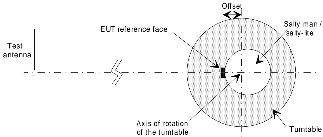
Figure 7: Illustration of offset from the axis of rotation
