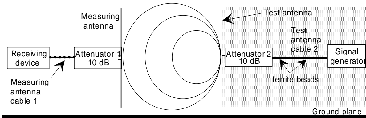
Figure 15: Stage 1: transform factor
