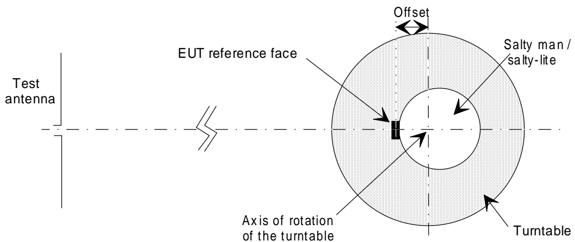
Figure 12: Illustration of offset from the axis of rotation
