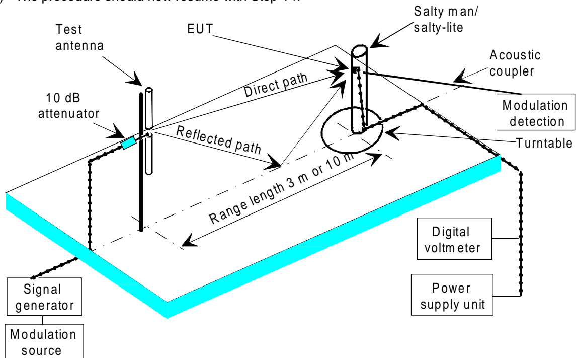
Figure 19: Open area test site set-up for sensitivity tests on the EUT
