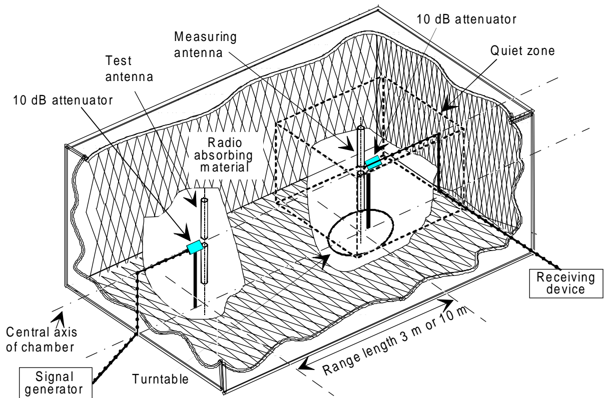
Figure 8: Equipment layout for the derivation of the transform factor during Sensitivity tests in an anechoic chamber
