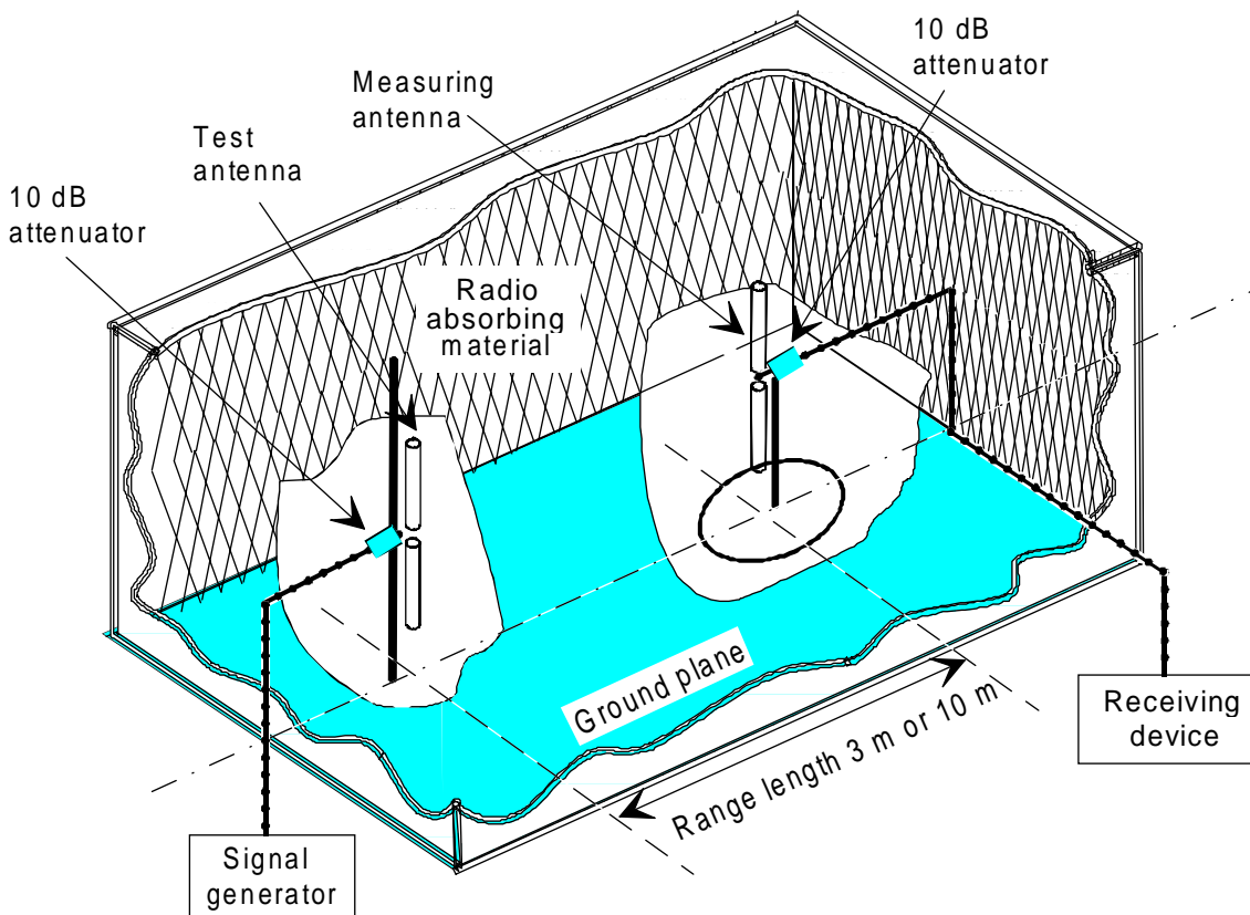
Figure 13: Equipment layout for the derivation of the transform factor during receiver sensitivity tests in an anechoic chamber with a ground plane
