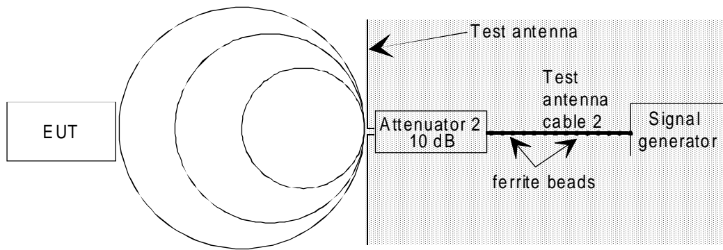
Figure 11: Stage 2: EUT measurement
