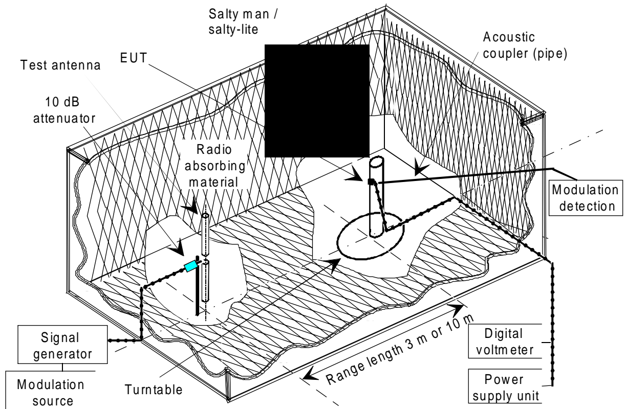
Figure 9: Anechoic chamber set-up for Sensitivity tests on the EUT
