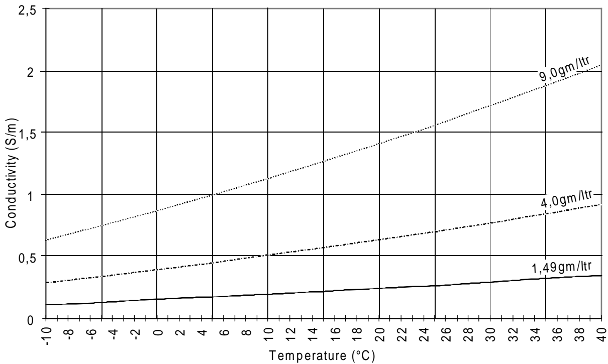
Figure 6: Variation of conductivity of various concentrations of saline solutions with temperature
