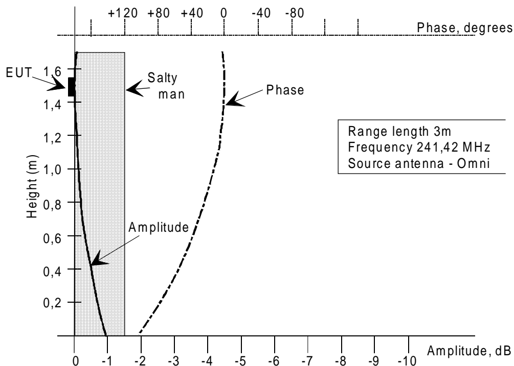
Figure 4: Amplitude and phase distribution along the Salty man over an absorptive ground
