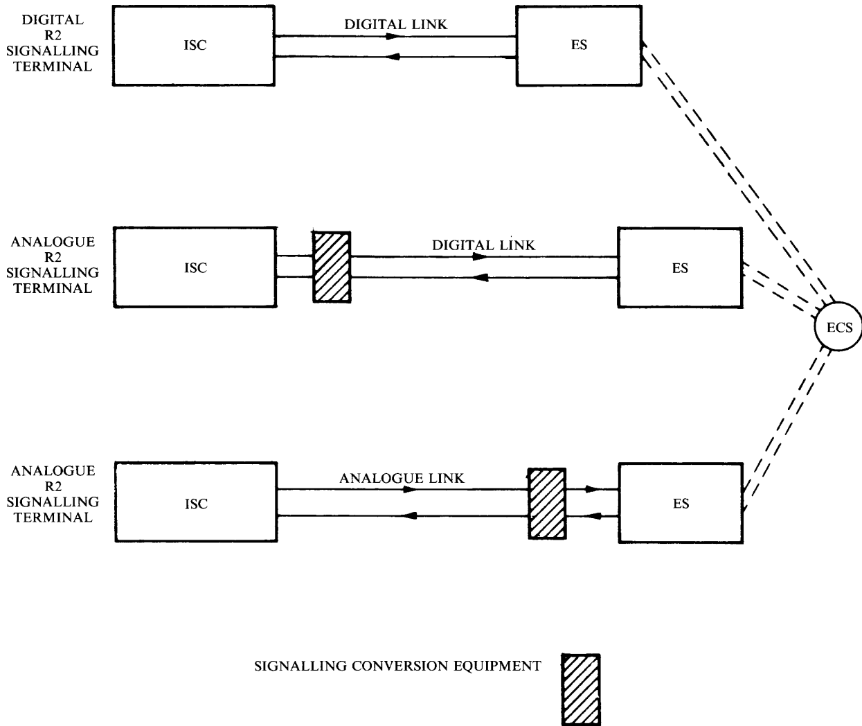
Figure 1 (T/CS 42-09). System R2 — ECS access configurations.
