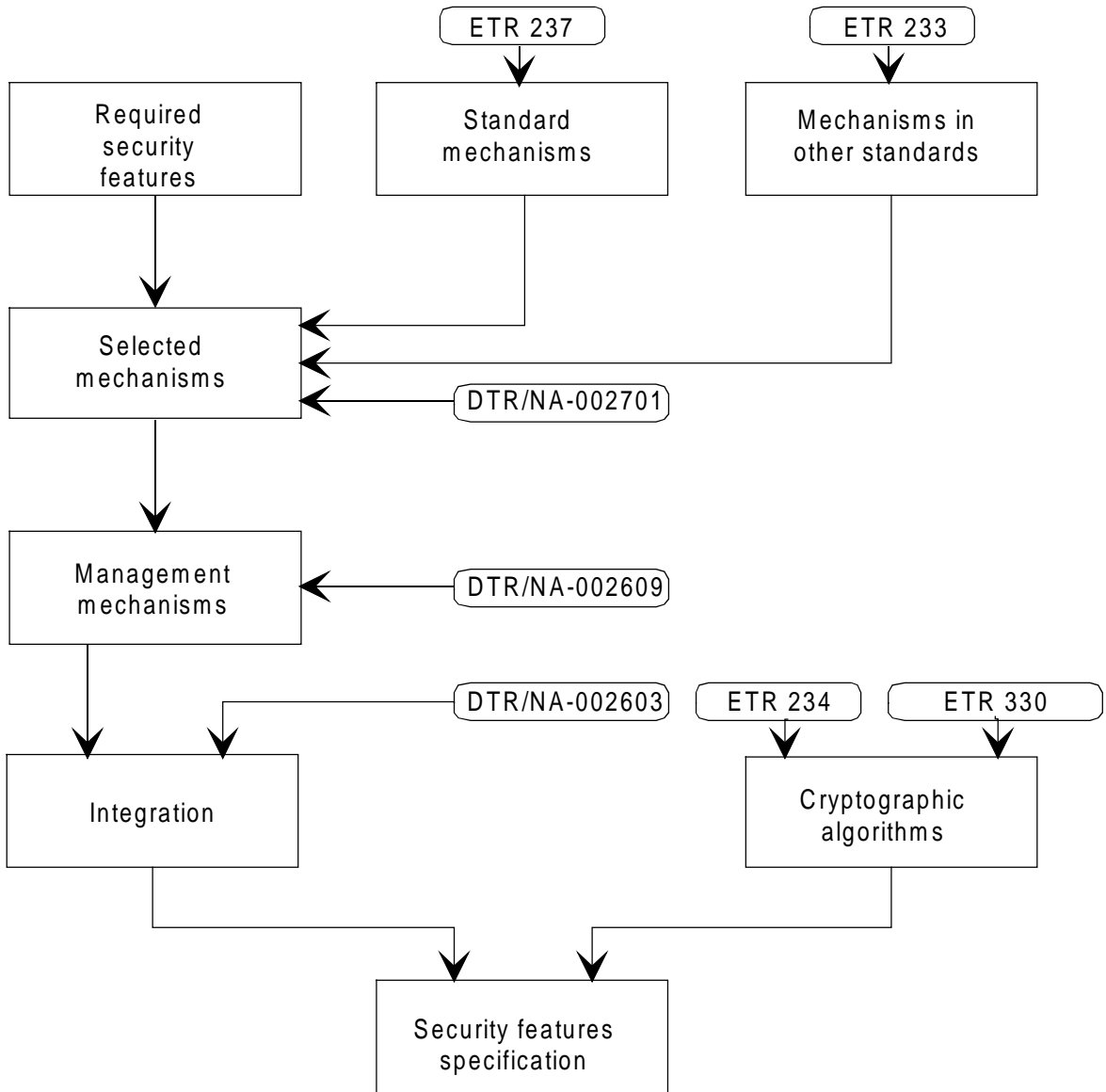
Figure 2: Specification of security features
