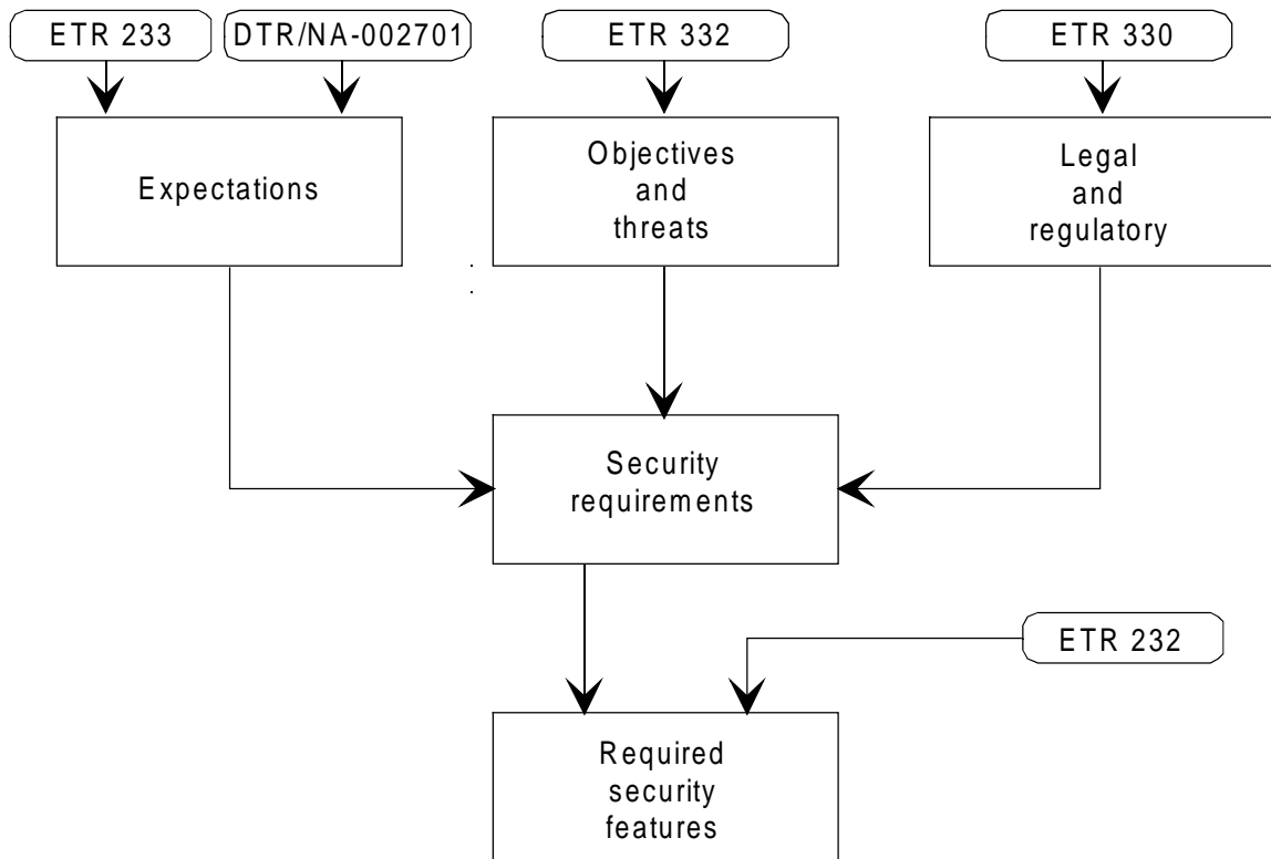
Figure 1: Capturing requirements for security features
