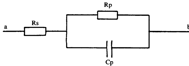
Figure 3 (T/STI 46-04). Impedance reference network (example).
