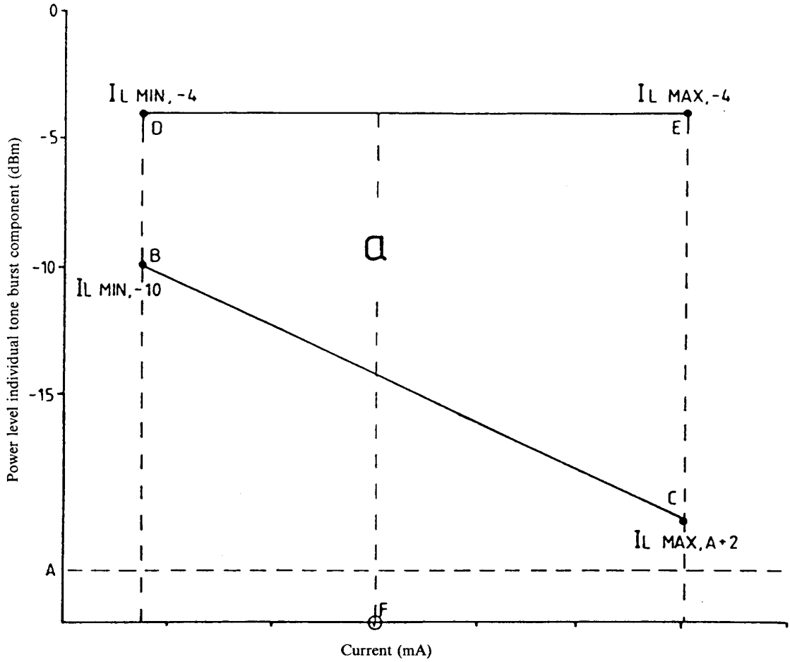
Figure 2B (T/STI 46-04). MF tone power levels regulated sender. OPTION 2.
