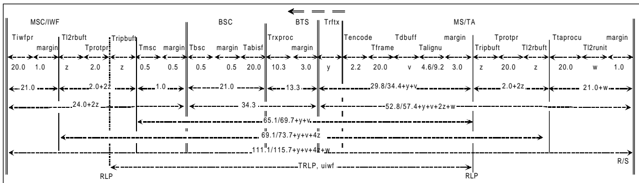
Fig 4/4b. Worst-case uplink delay distribution for data TCH (non-transparent data)
