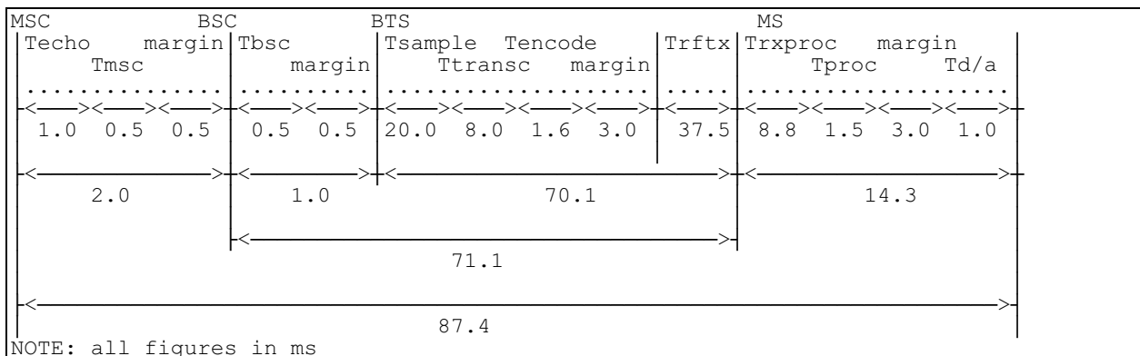
Fig 4/2a: Downlink delay distribution for TCH/FS (64 Kbit/s Abis)
