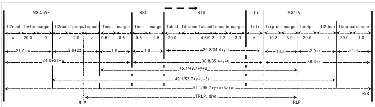
Fig 4/4a. Worst-case downlink delay distribution for data TCH (non-transparent data)
