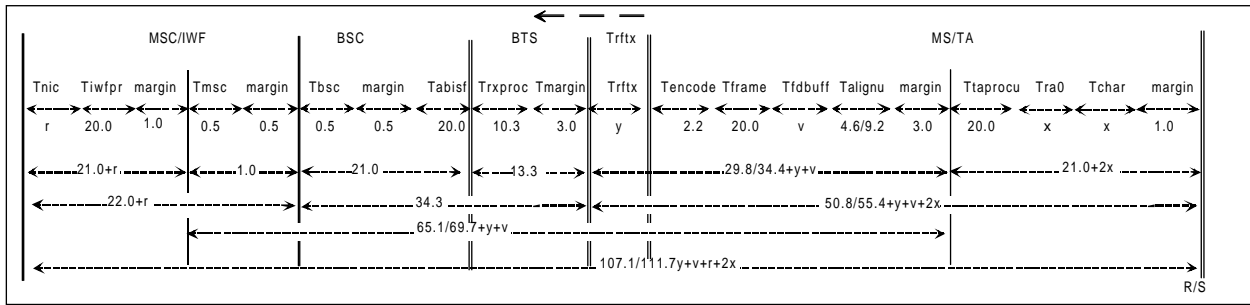
Fig 4/3b. Worst-case uplink delay distribution for data TCH (transparent data)
