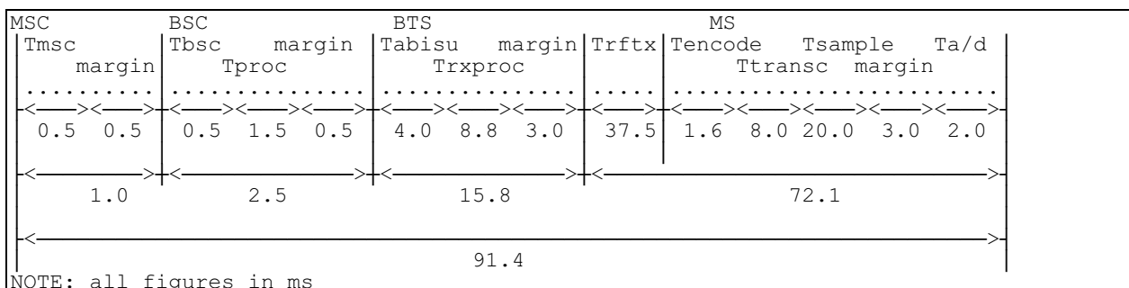
Fig 4/1b: Uplink delay distribution for TCH/FS (16 Kbit/s Abis)
