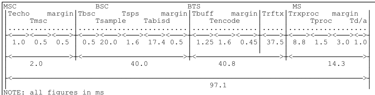
Fig 4/1a: Downlink delay distribution for TCH/FS (16 Kbit/s Abis)
