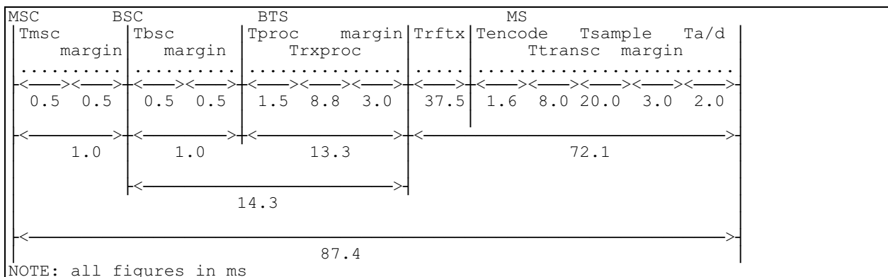
Fig 4/2b: Uplink delay distribution for TCH/FS (64 Kbit/s Abis)
