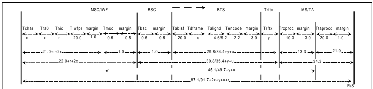
Fig 4/3a. Worst-case downlink delay distribution for data TCH (transparent data)
