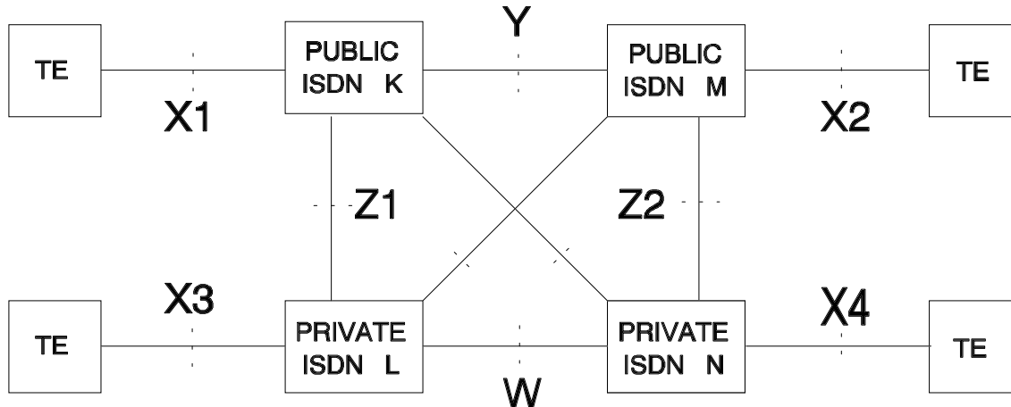
Figure E.1 1) : Access and interconnection points in ISDN concept
