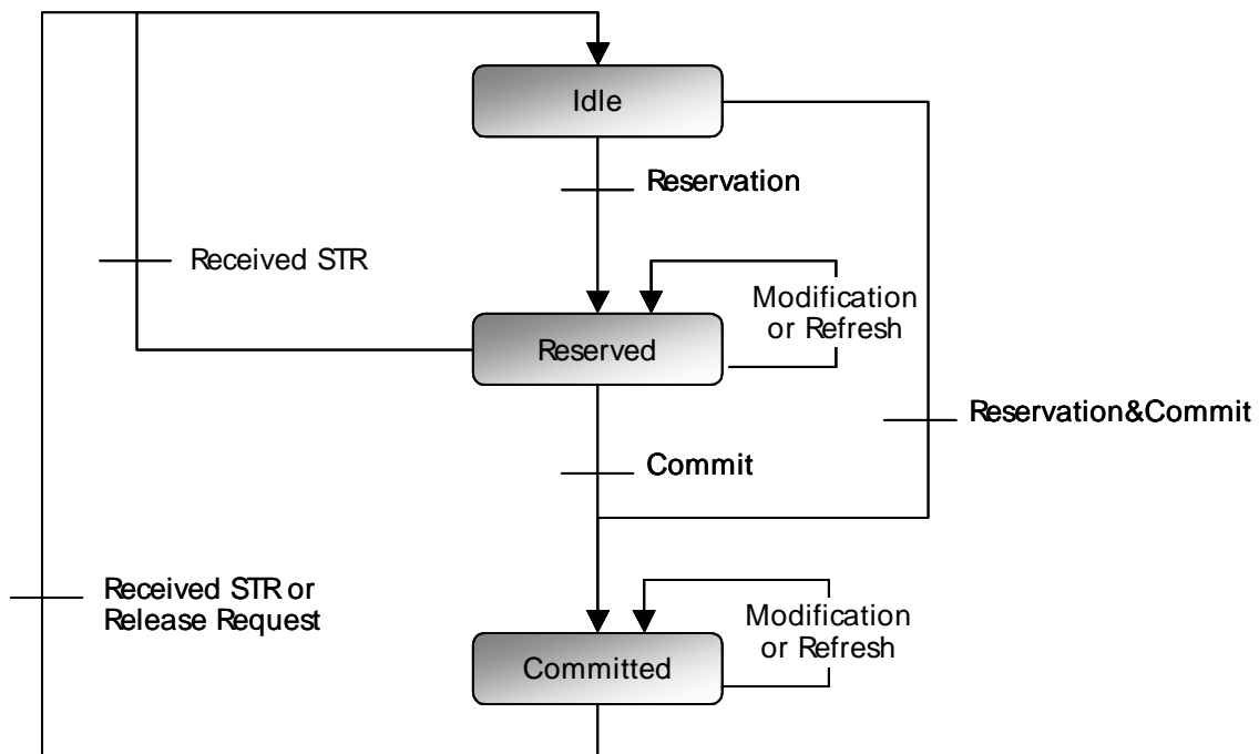
Figure 2: Flow state
