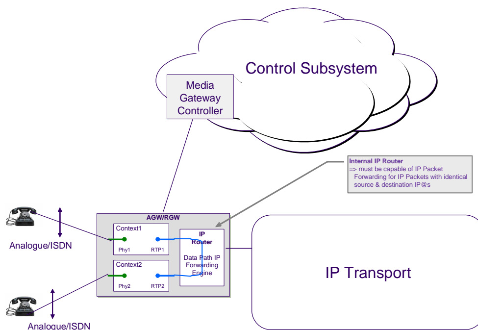
Figure 2: Single RTP session - internal bearer redirection via embedded IP router
