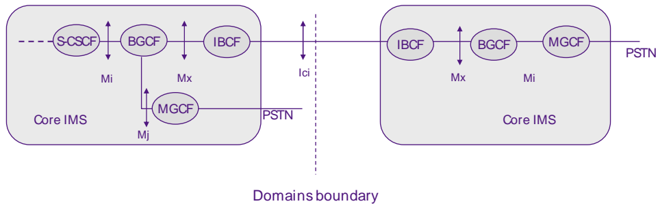
Figure B.4: IMS session with PSTN interworking
