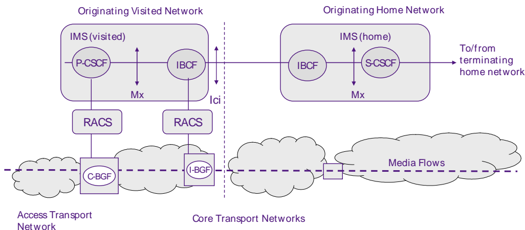
Figure 6: IMS interconnect scenario with I-BGF
