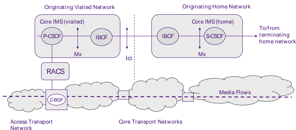
Figure 5: IMS interconnect scenario without I-BGF
