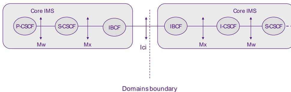
Figure B.2: IMS session between two networks
