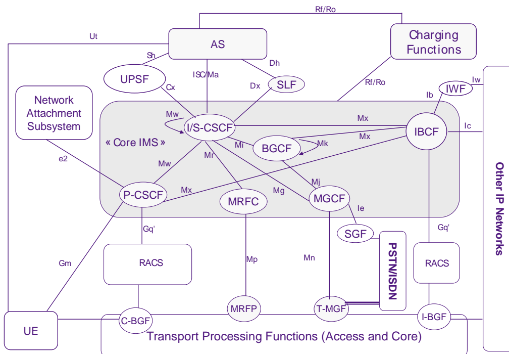
Figure 3: NGN IMS overview
