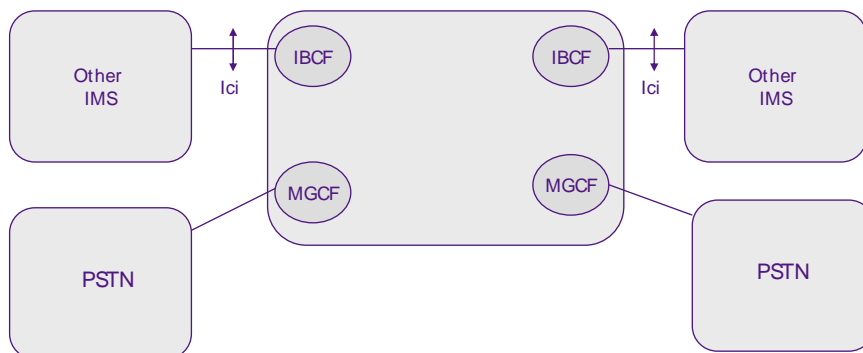
Figure B.7: IMS transit scenarios
