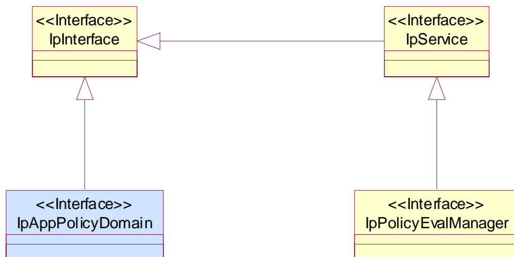
Figure 3: Policy Evaluation Classes
