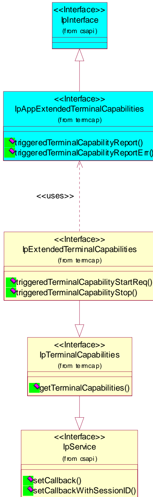
Figure 1: Terminal Capabilities Class Diagram
