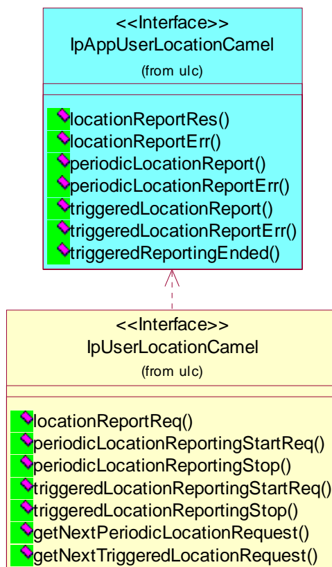
Figure 2: User Location Camel Class Diagram
