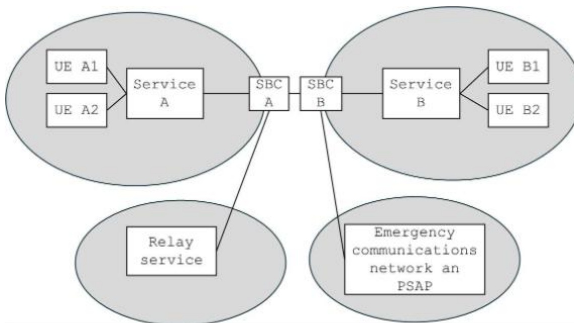
Figure 5.1: Conceptual view of a total conversation service architecture
