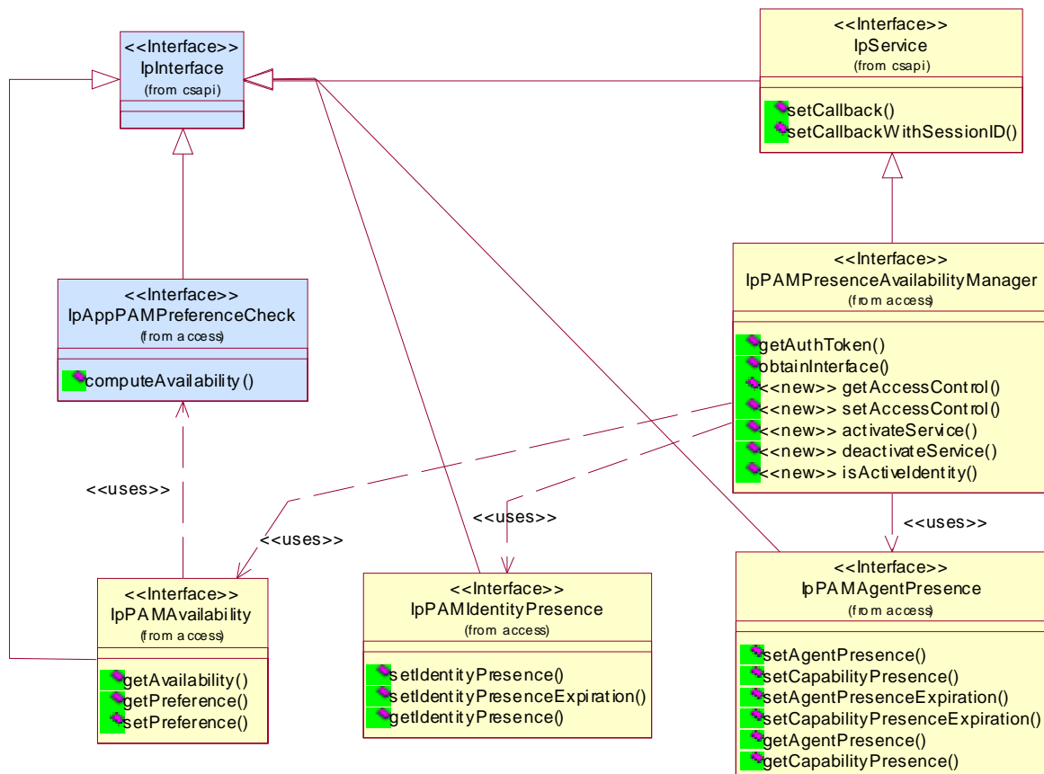
Figure 2: PAM Access Service
