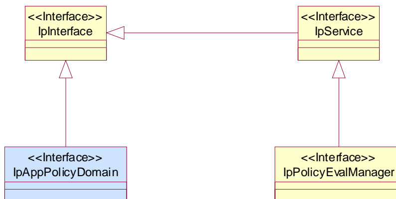
Figure 3: Policy Evaluation Classes
