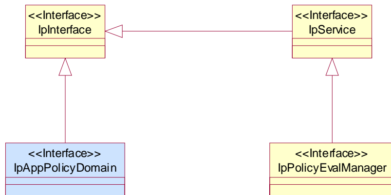
Figure 3: Policy Evaluation Classes
