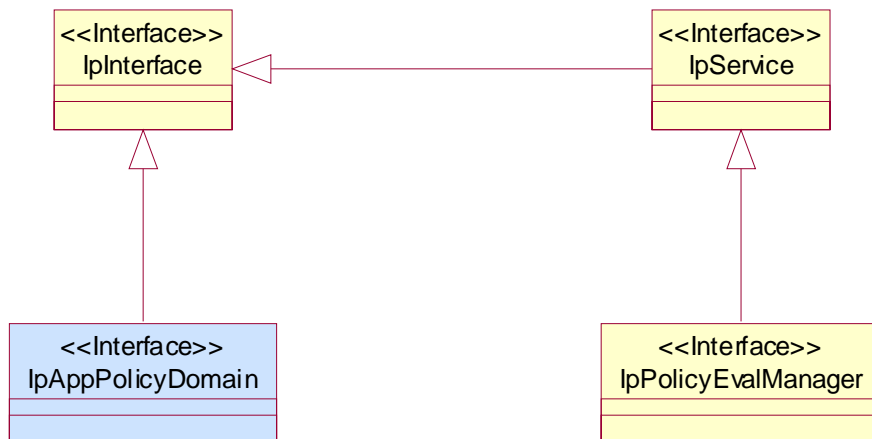
Figure 3: Policy Evaluation Classes
