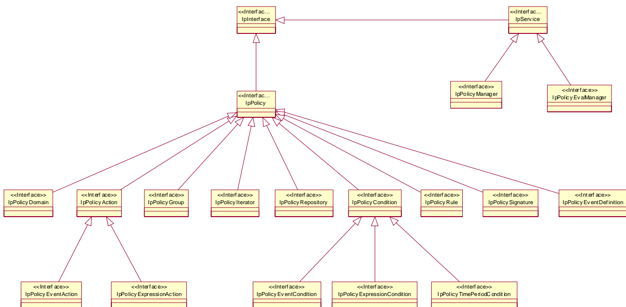
Figure 1: Policy Provisioning Classes
