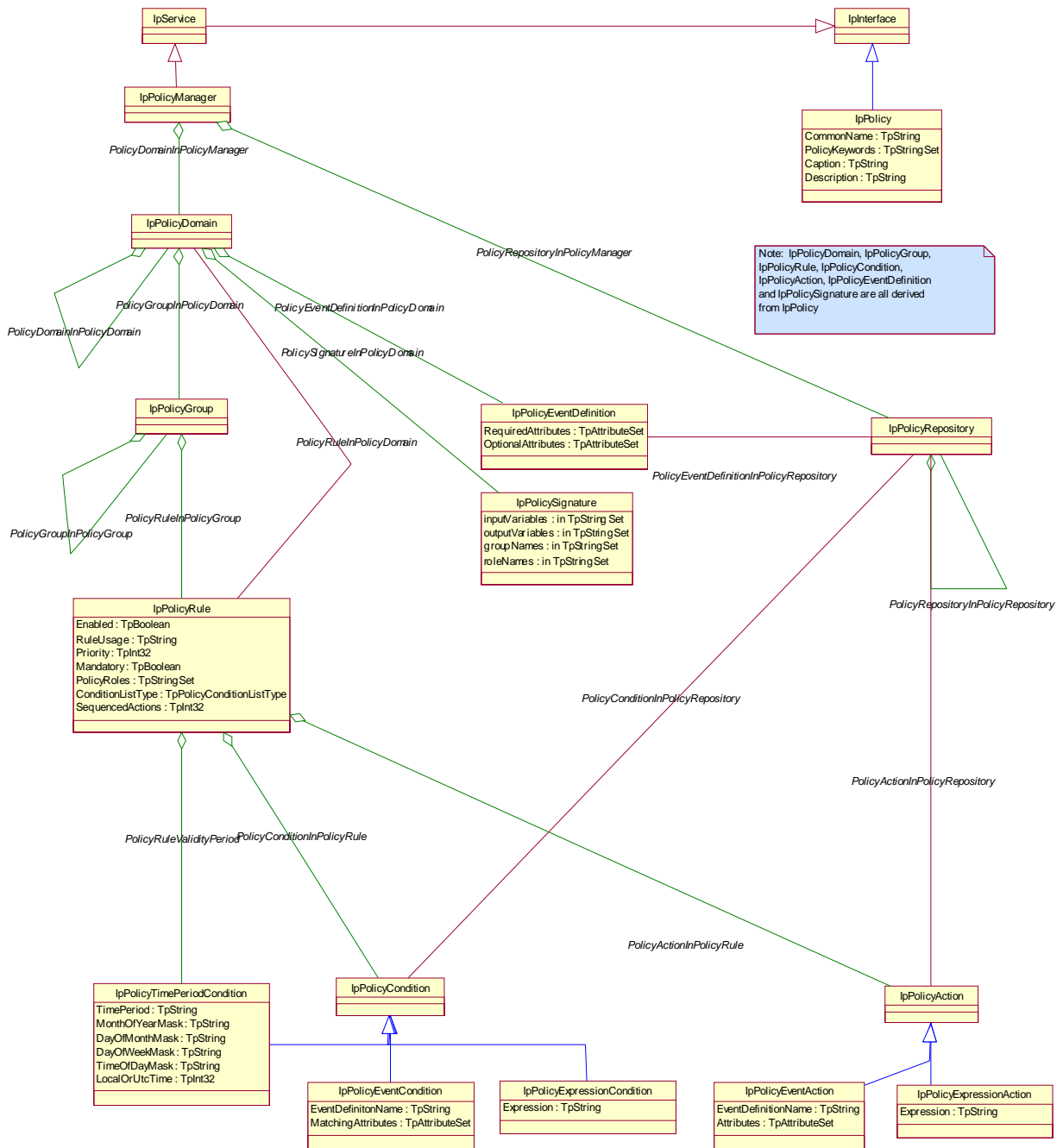
Figure 2: Policy Management Information Model
