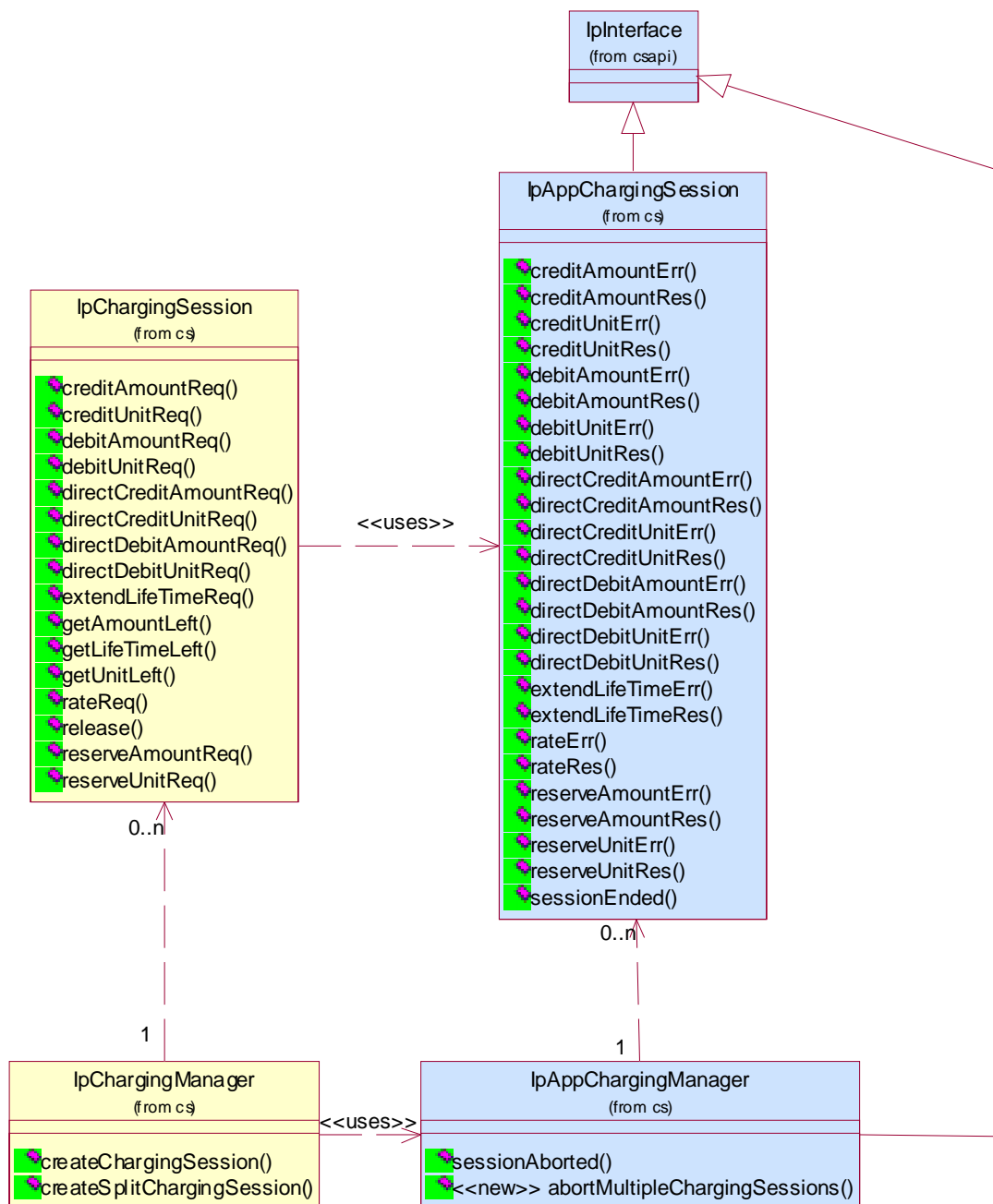
Figure 1: Application Interfaces
