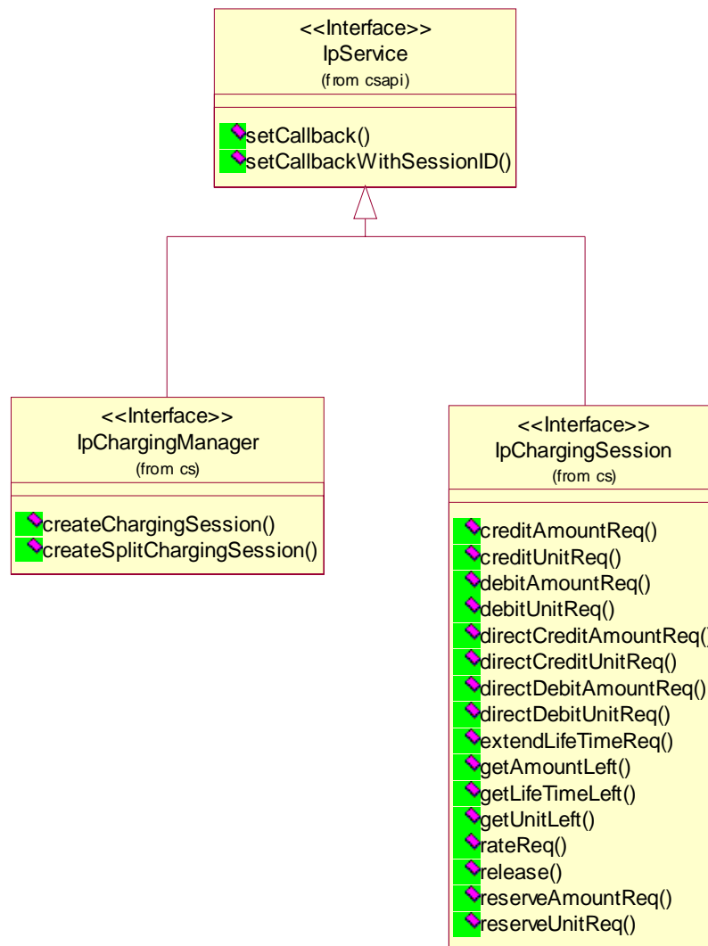
Figure 2: Service Interfaces
