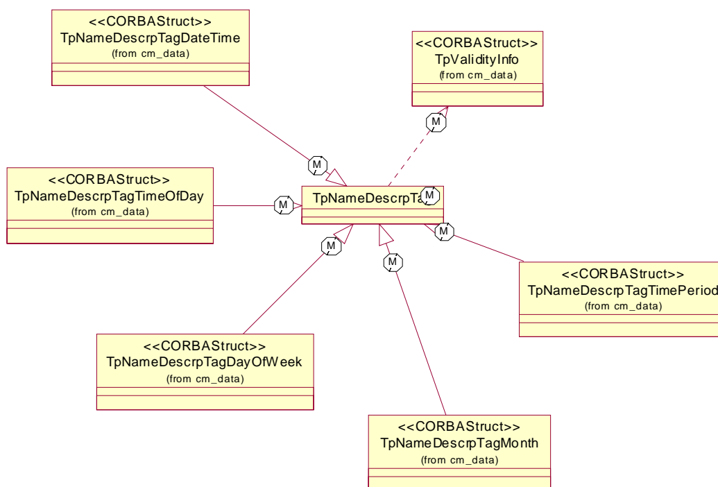
Figure 7: Validity Data Type Classes
