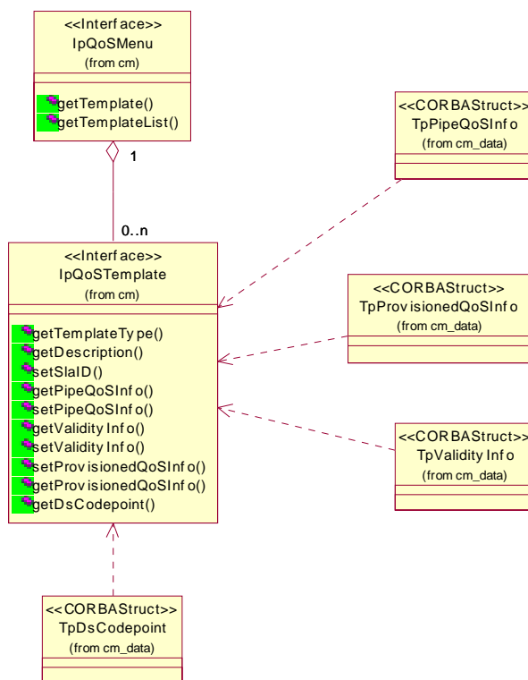
Figure 3: QoS Template class diagram
