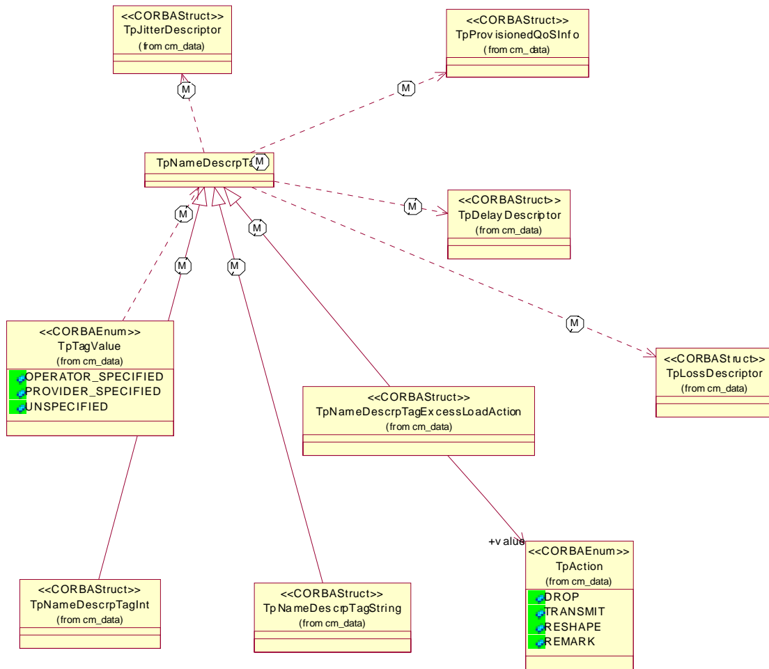
Figure 4: Provisioned QoS Data Types Classes
