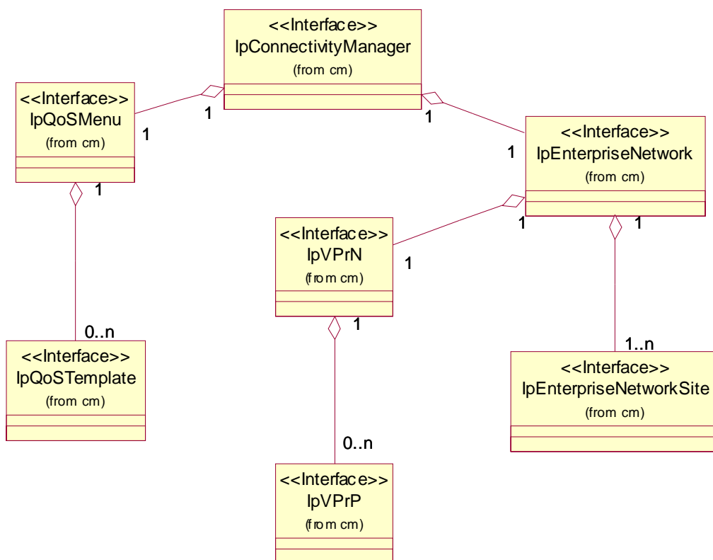
Figure 1: Connectivity Management High level class diagram
