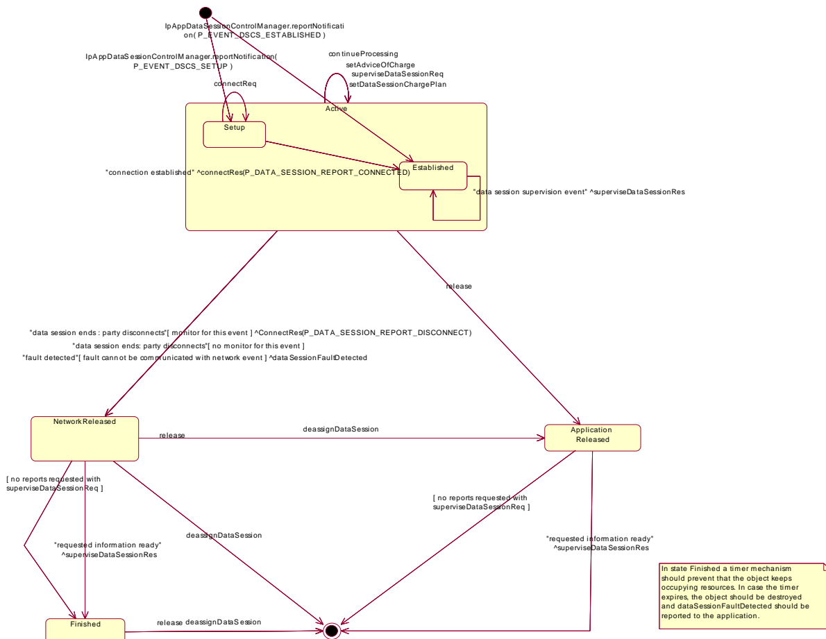
Figure 3: Application view on the Data Session object
