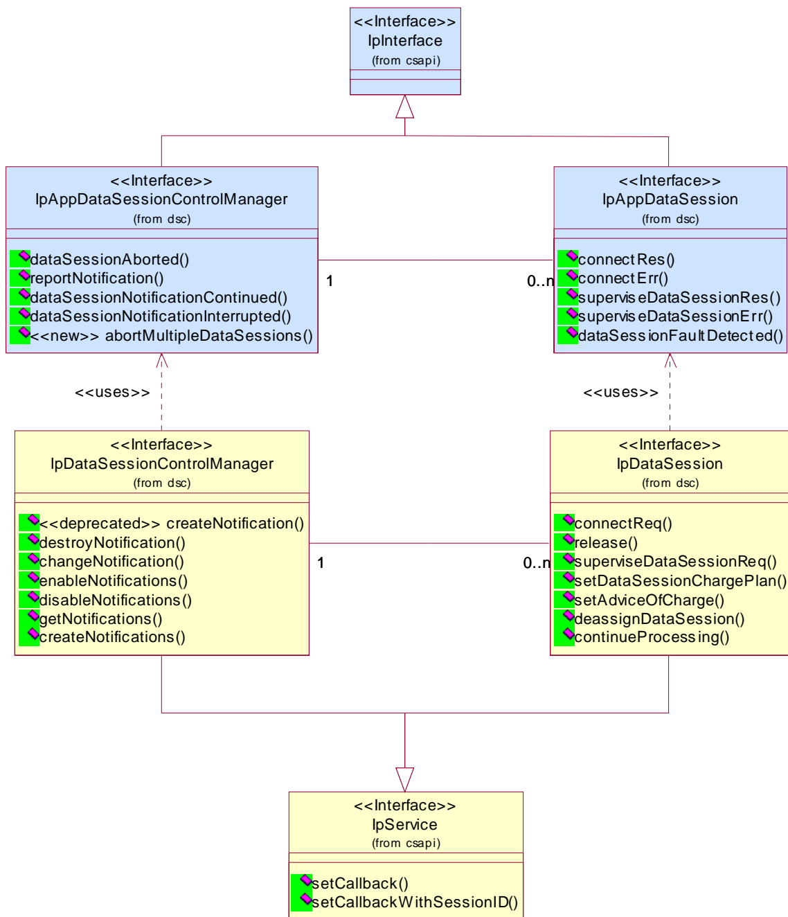
Figure 2: Package Overview
