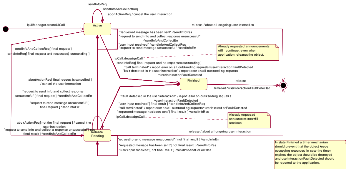
Figure 5: Application view on the UICall object
