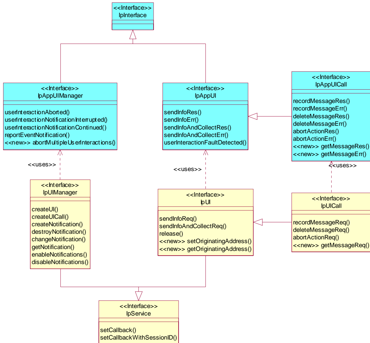
Figure 1: Generic User Interaction Package Overview
