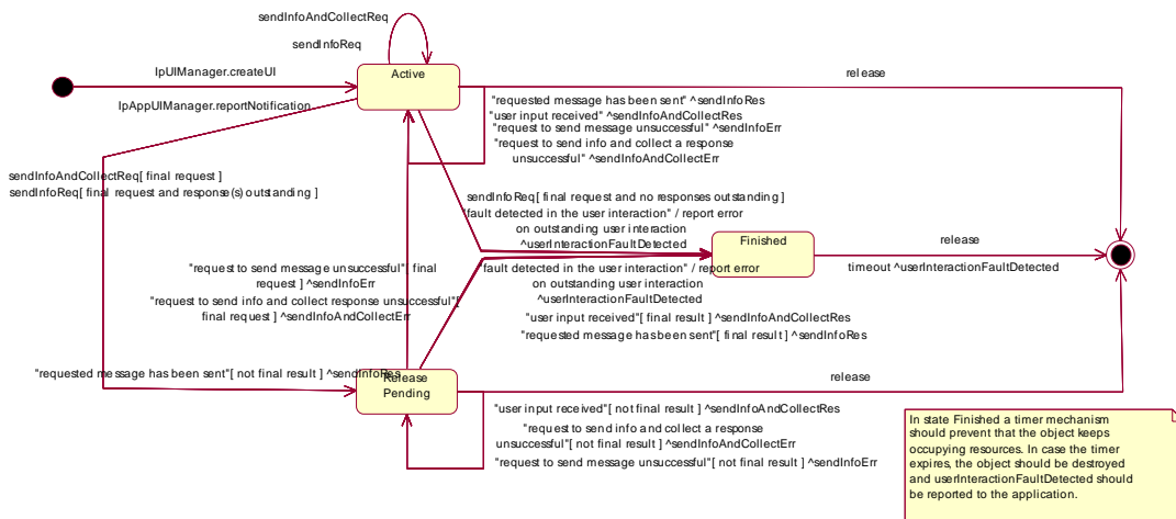
Figure 4: Application view on the UI object
