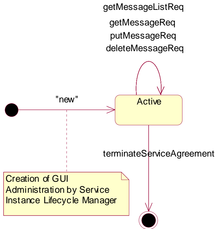
Figure 6: State Transition Diagram for User Interaction Administration
