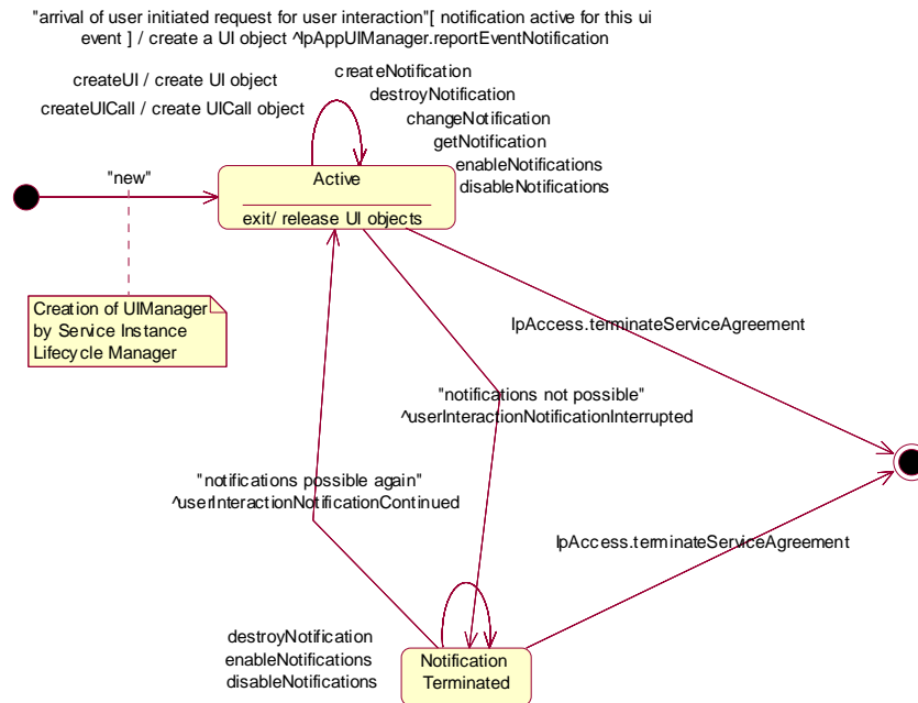
Figure 3: Application view on the UI Manager
