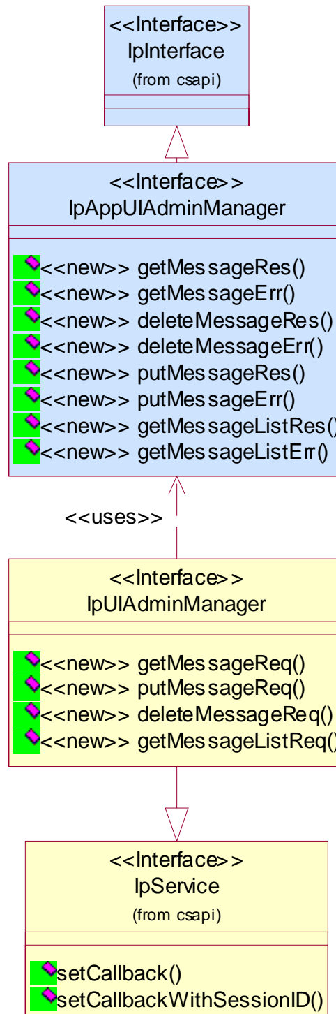
Figure 2: Generic User Administration Package Overview
