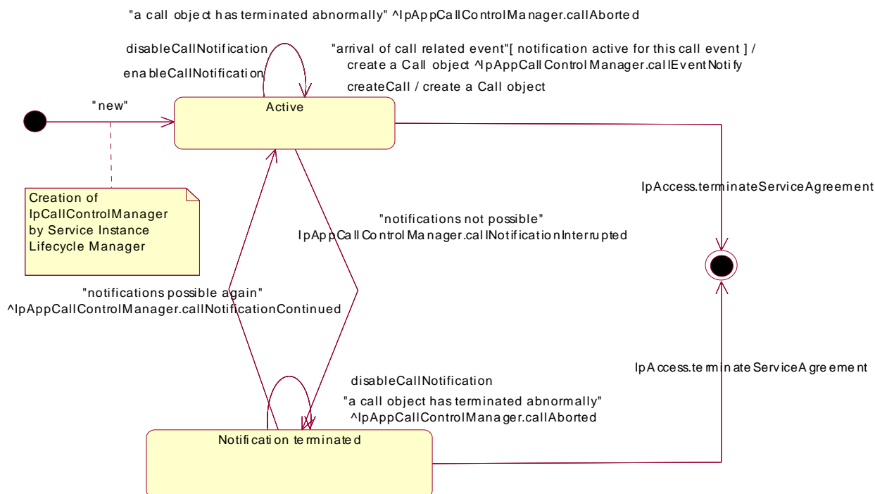
Figure 3: Application view on the Call Control Manager
