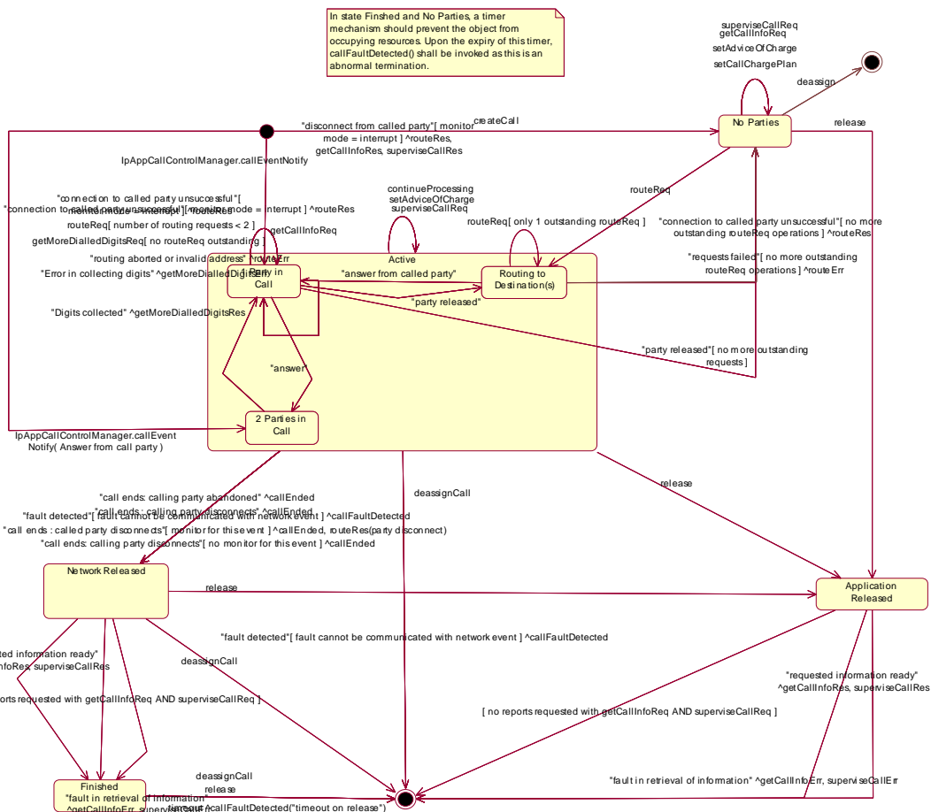
Figure 4: Application view on the IpCall object
