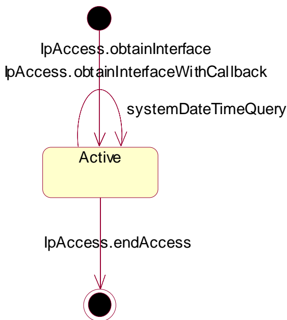
Figure 16: State Transition Diagram for IpOAM
