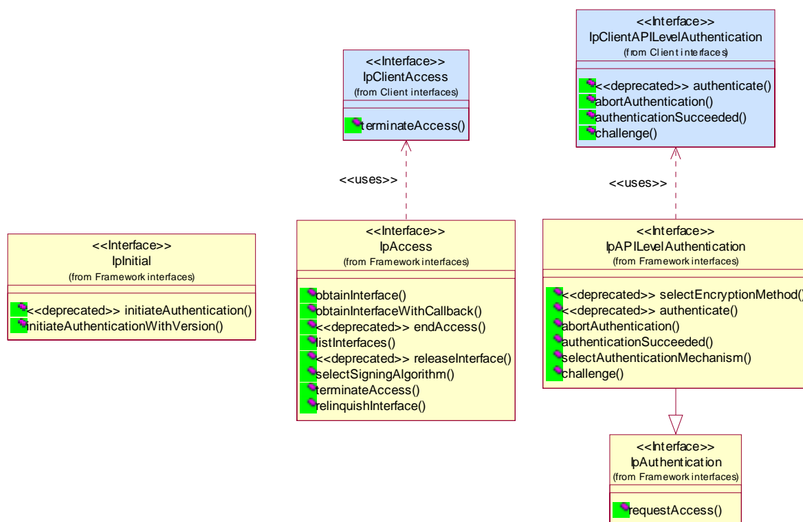
Figure 31: Trust and Security Management Package Overview
