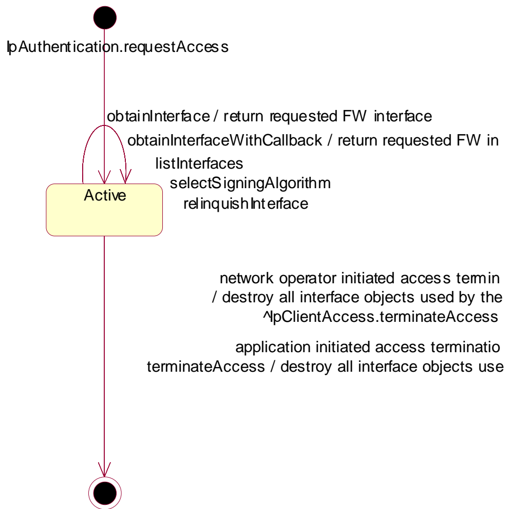
Figure 7: State Transition Diagram for IpAccess
