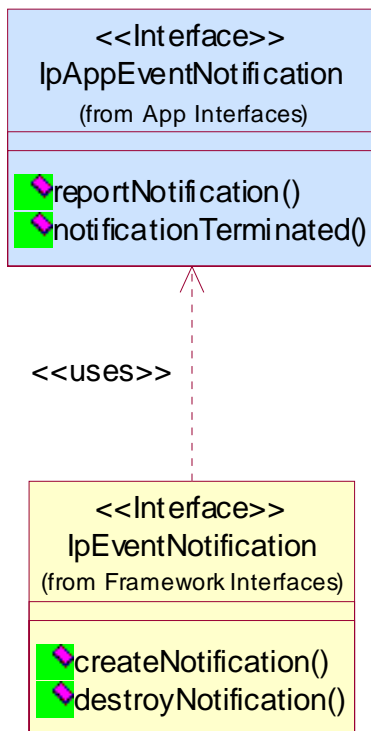
Figure 8: Event Notification Class Diagram
