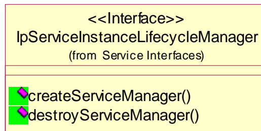
Figure 29: Service Instance Lifecycle Manager Package Overview
