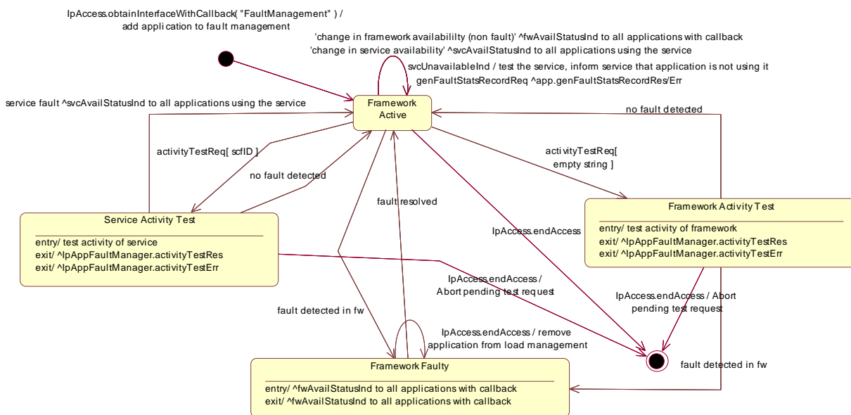
Figure 17: State Transition Diagram for IpFaultManager
