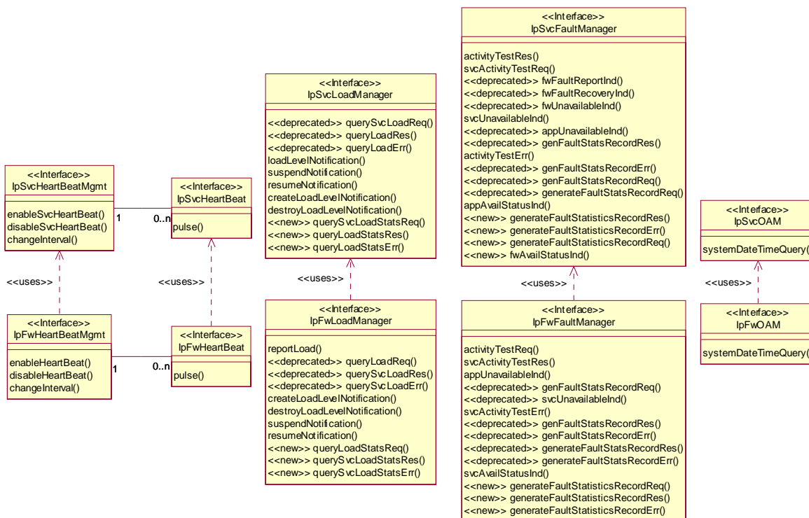
Figure 27: Integrity Management Package Overview
