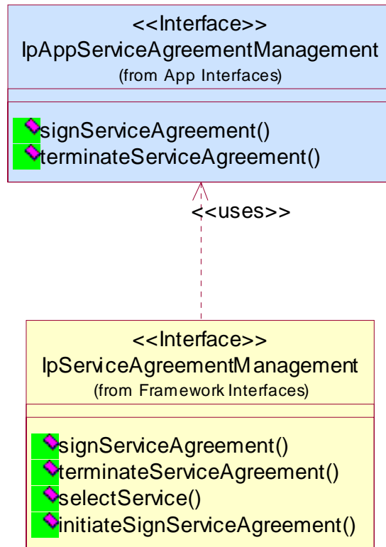
Figure 10: Service Agreement Management Package Overview
