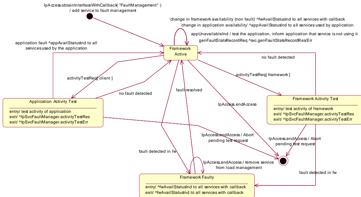
Figure 34: State Transition Diagram for IpFwFaultManager
