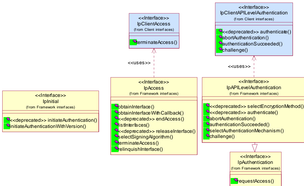
Figure 12: Trust and Security Management Package Overview
