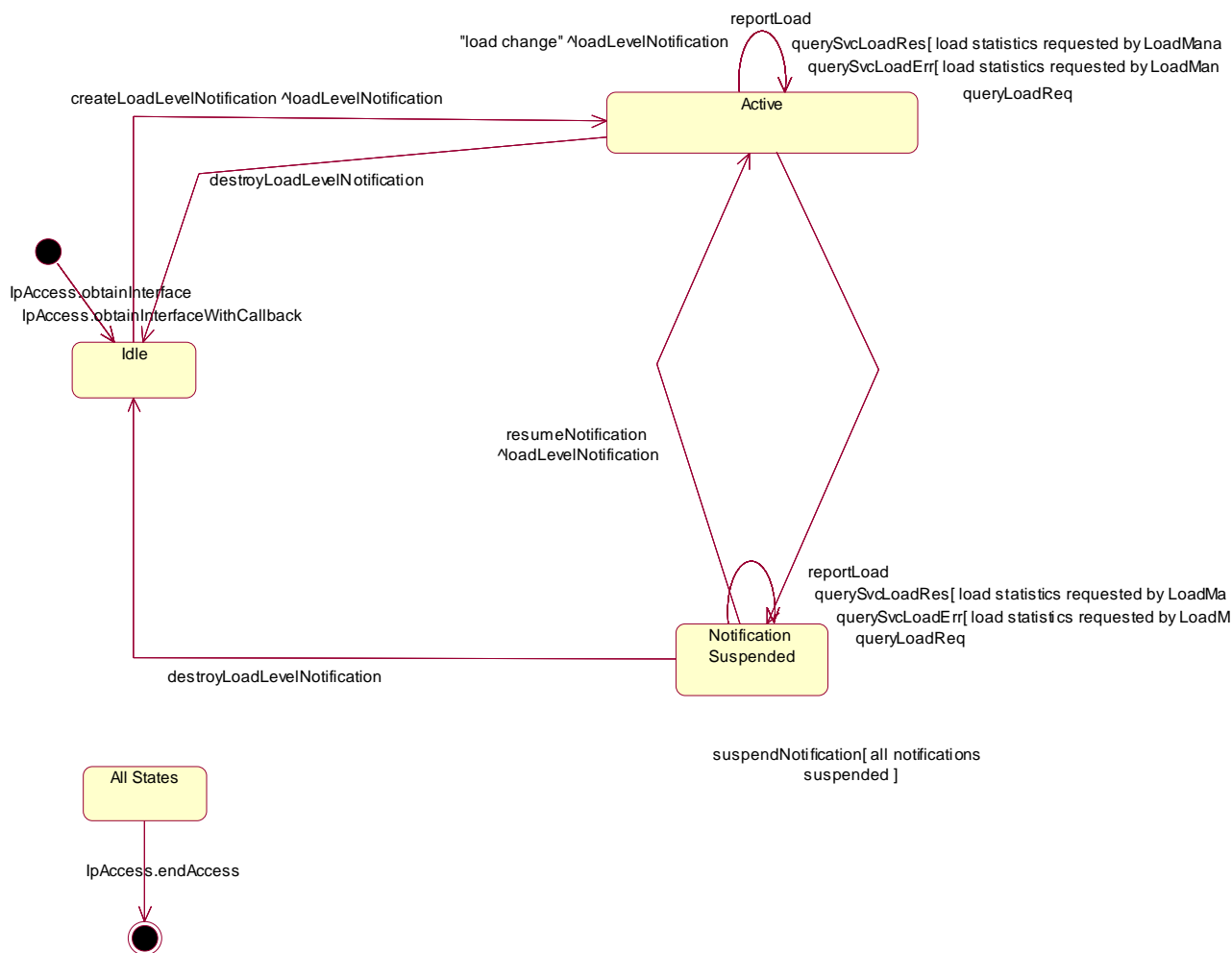
Figure 14: State Transition Diagram for IpLoadManager
