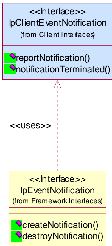
Figure 23: Event Notification Package Overview
