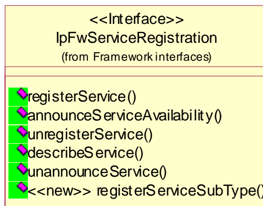
Figure 30: Service Registration Package Overview
