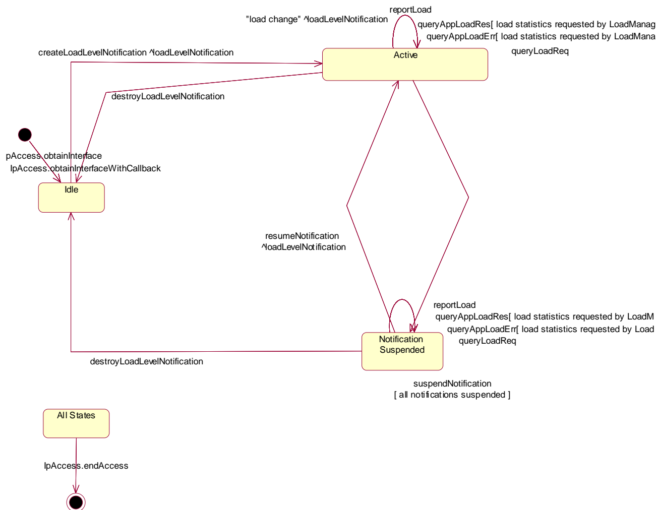
Figure 33: State Transition Diagram for IpFwLoadManager
