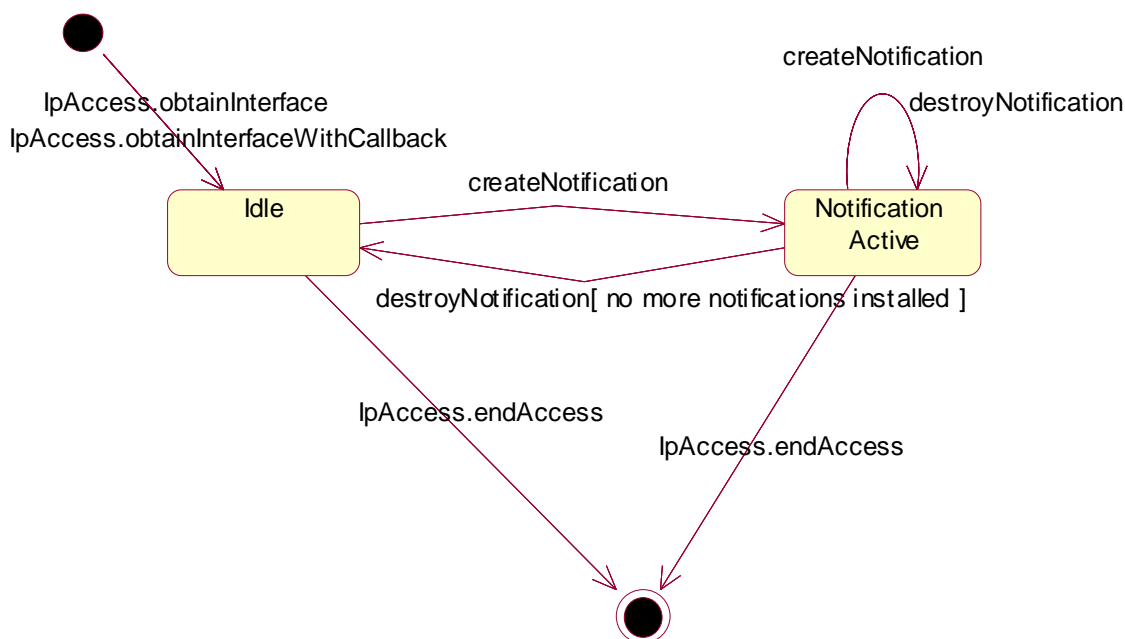
Figure 18: State Transition Diagram for IpEventNotification
