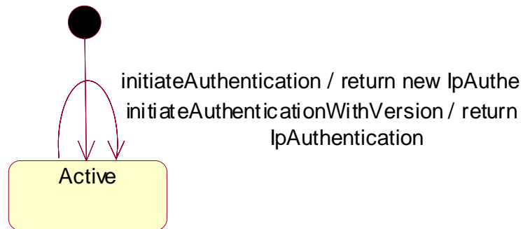
Figure 2: State Transition Diagram for IpInitial
