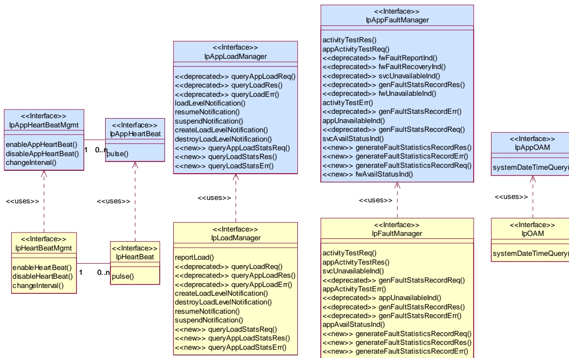
Figure 9: Integrity Management Package Overview
