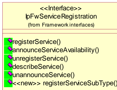
Figure 31: Service Registration Package Overview
