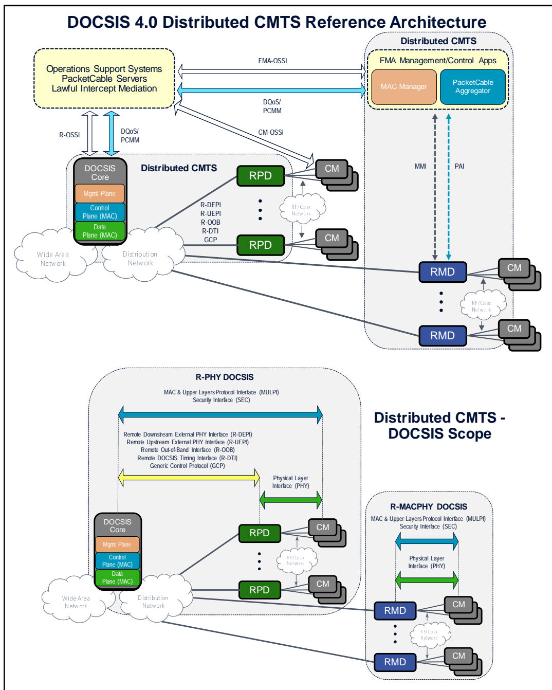
Figure 3: Distributed CMTS reference architecture
