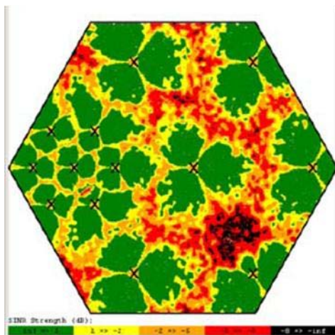
Figure 2: Typical SINR distribution of a mobile network
