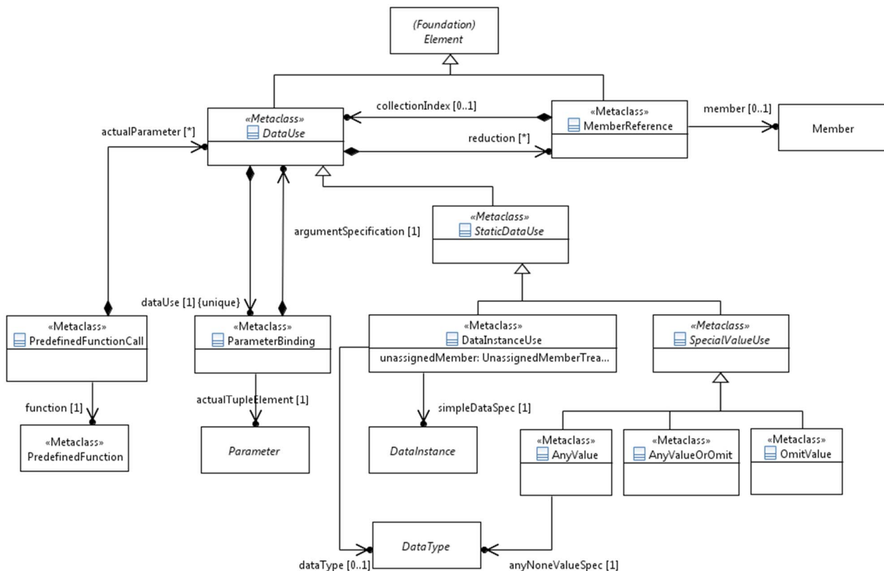
Figure 6.7: Data use concepts and static data use
