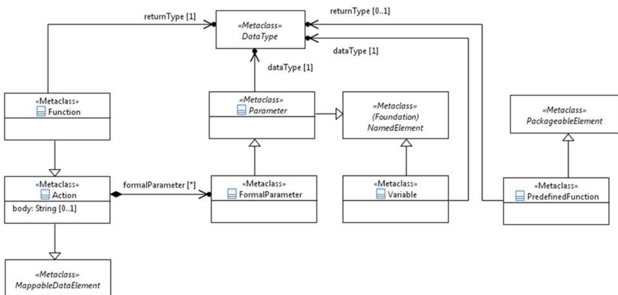
Figure 6.6: Action, function, parameter and variable
