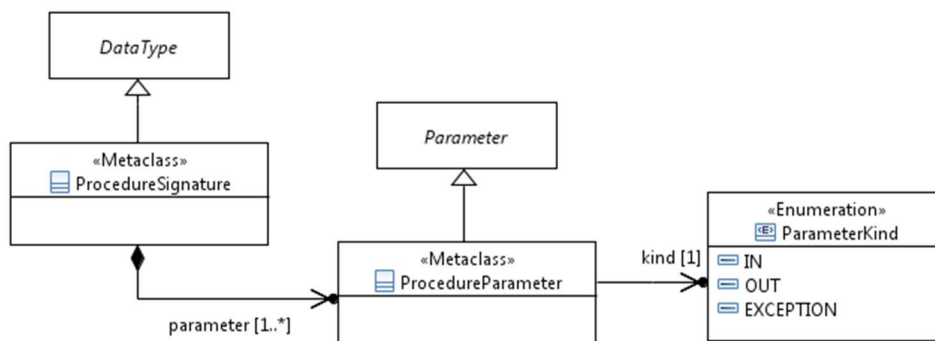
Figure 6.5: Procedure and procedure parameter
