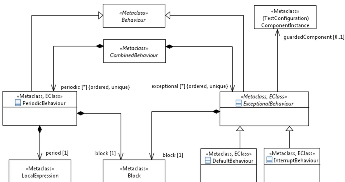
Figure 9.3: Exceptional and periodic behaviour
