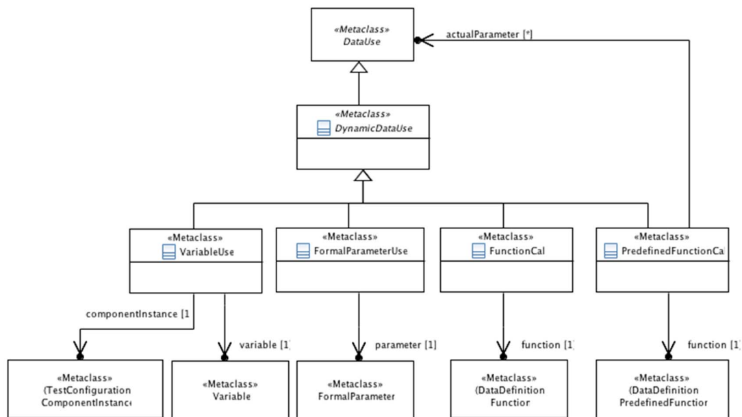
Figure 6.8: Dynamic data use
