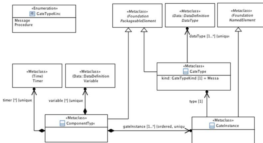
Figure 8.1: Component and gate type
